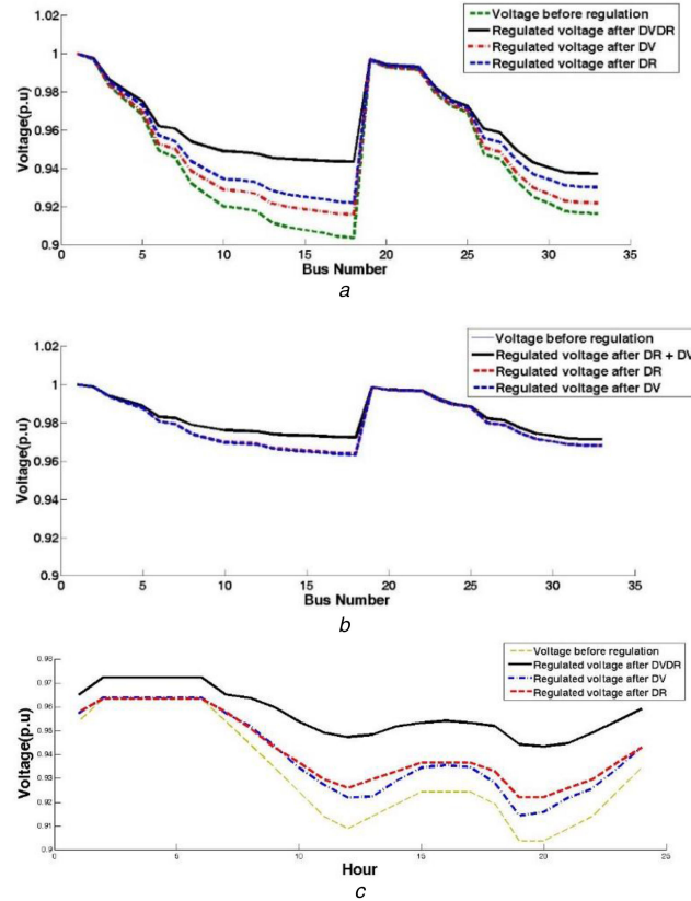
Fig. 7 Voltage amount before and after voltage regulation at hour 20 (maximum load factor), 2 (minimum load factor) and 24 h in Scenario 2 (a) Hour 20 (maximum load factor), (b) Hour 2 (minimum load factor), (c) 24 h
