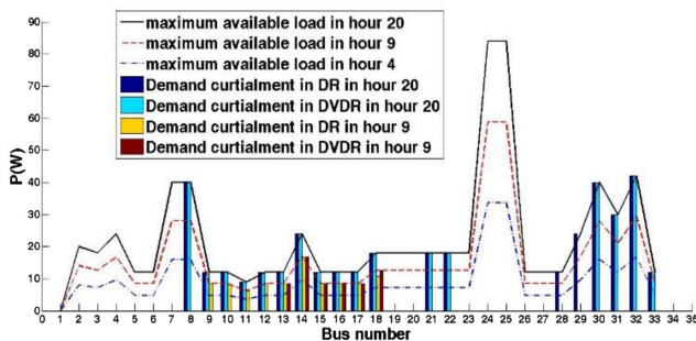
Fig. 6 Demand curtailment using DR and DVDR methods in Scenario 1
