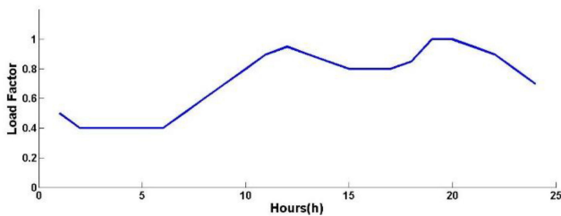
Fig. 3 Load factor at each time
