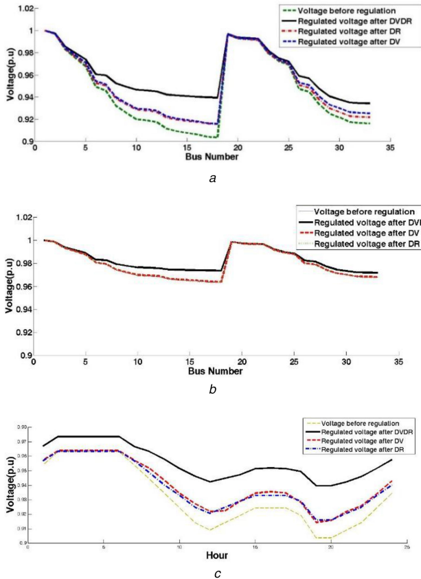
Fig. 5 Voltage amount before and after voltage regulation at hour 20 (maximum load factor), hour 2 (minimum load factor) and 24 h in Scenario 1
