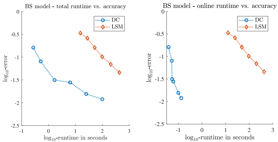
Figure 5.5: Log-Log plot of the total/online runtime vs. accuracy. Comparison of the Dynamic Chebyshev method with the Least-Square Monte-Carlo algorithm.
