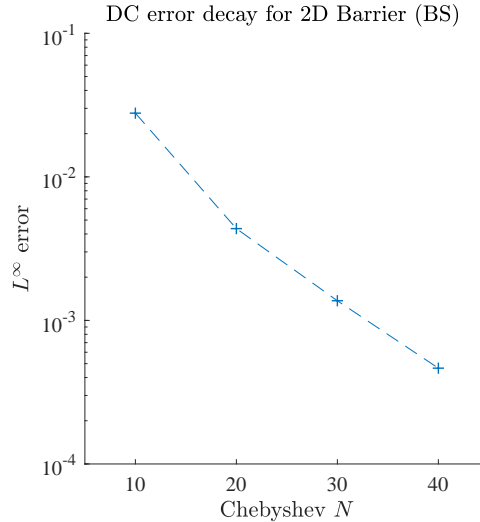
Figure 5.3: Error decay of the Dynamic Chebyshev approach for a bivariate barrier option in a multivariate BS model. The conditional expectation of the Chebyshev polynomials are calculated using the density function.
