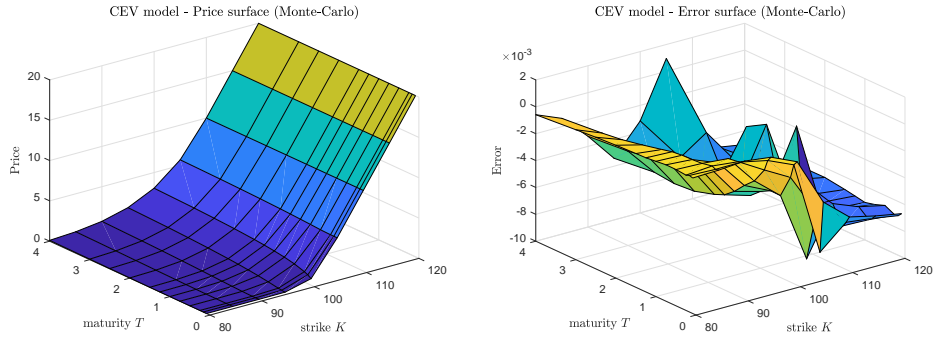
Figure 5.7: Price surface and corresponding error of the Dynamic Chebyshev method in the CEV model. The conditional expectations are calculated with Monte-Carlo.
