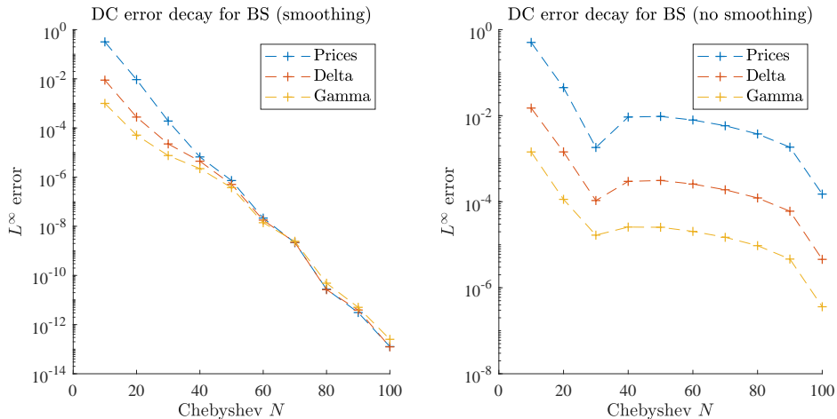
Figure 5.1: Error decay prices Dynamic Chebyshev in the BS model using smoothing in the first time step(left) and without smoothing (right). The conditional expectation of the Chebyshev polynomials are calculated with the density function.
