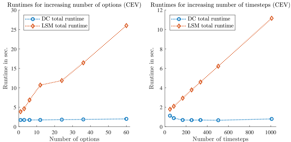
Figure 5.9: Total runtime of the DC and the LSM method for an increasing number of options (left) and an increasing number of timesteps (right).
