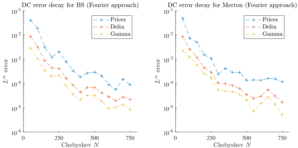
Figure 5.2: Error decay prices Dynamic Chebyshev in the BS model (left) and the Merton model (right). The conditional expectation of the Chebyshev polynomials are calculated with the Fourier transformation.
