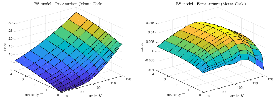
Figure 5.4: Price surface and corresponding error of the Dynamic Chebyshev method in the Black-Scholes model. The conditional expectations are calculated with Monte-Carlo.
