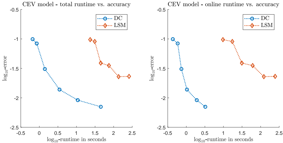
Figure 5.8: Log-Log plot of the total/online runtime vs. accuracy. Comparison of the Dynamic Chebyshev method with the Least-Square Monte-Carlo algorithm.
