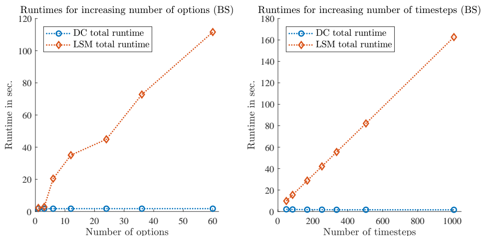
Figure 5.6: Total runtime of the DC and the LSM method for an increasing number of options (left) and an increasing number of timesteps (right).
