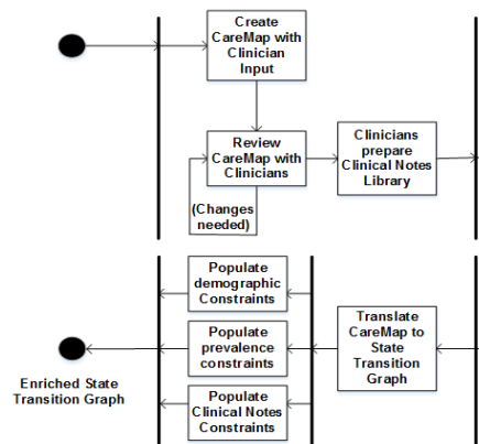
Fig. 8. UML Activity Diagram: Process of creating and integrating constraints into State Transition Machine for the midwifery Caremap.
