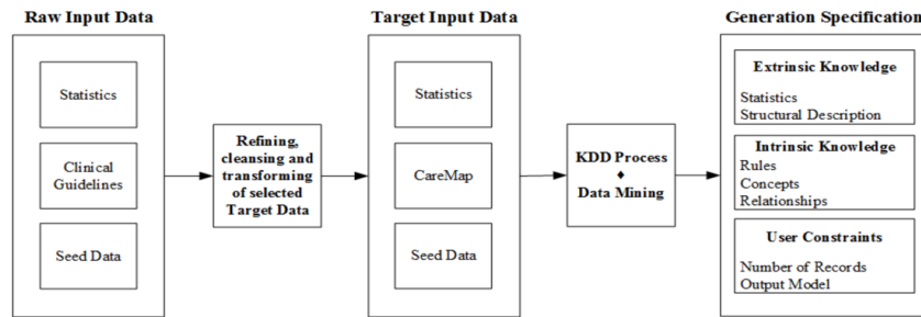
Fig. 3. Overview of the RA approach to realism in SDG
