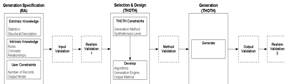
Fig. 4. HORUS approach to realism validation, showing touch points with THOTH and RA
