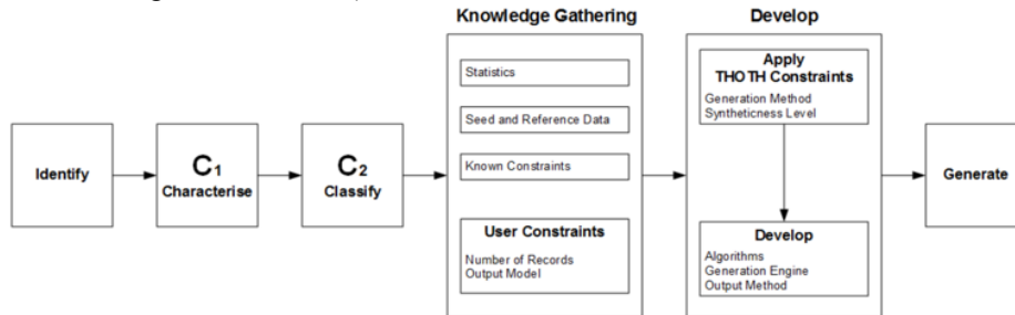
Fig. 2. THOTH integrated into the generic approach to SDG
