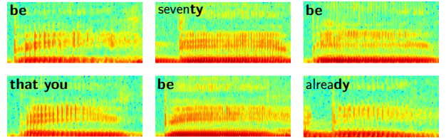
Figure 3: Spectrograms for random tokens from the cluster of ES-KMeans mapped to “be” in Figure 2. The portion of each true word which is covered by the segment is shown in bold.
