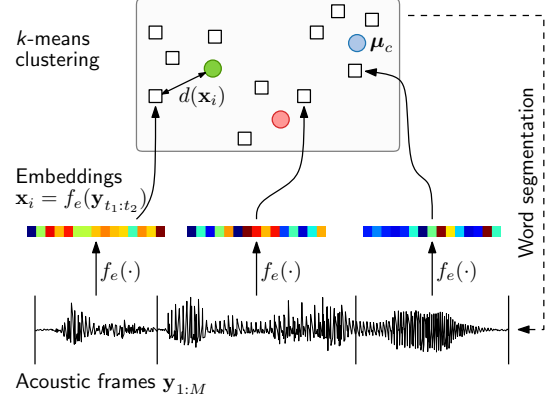
Figure 1: The embedded segmental k -means model for unsupervised segmentation and clustering of speech.
