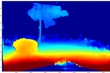
(e) DispNet
