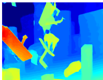
(g) Supervised 1
