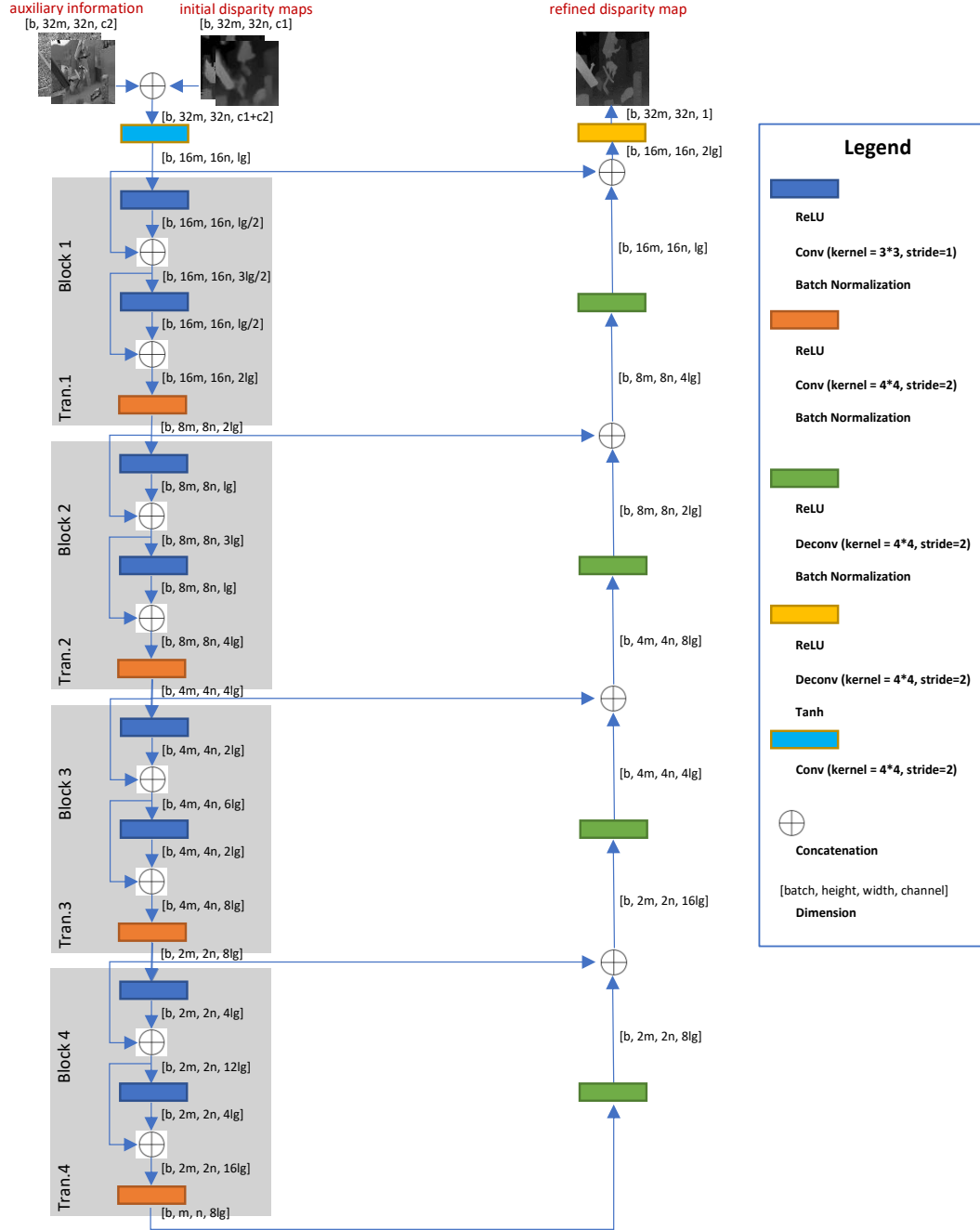
Figure 2: This figure shows some important hyperparameters and the refiner architecture configuration. Please refer to Table 2 for the specific values in each experiment. Tip: Readers can deepen the refiner by symmetrically adding more dense blocks and deconvolution layer by themselves according to their own needs.
