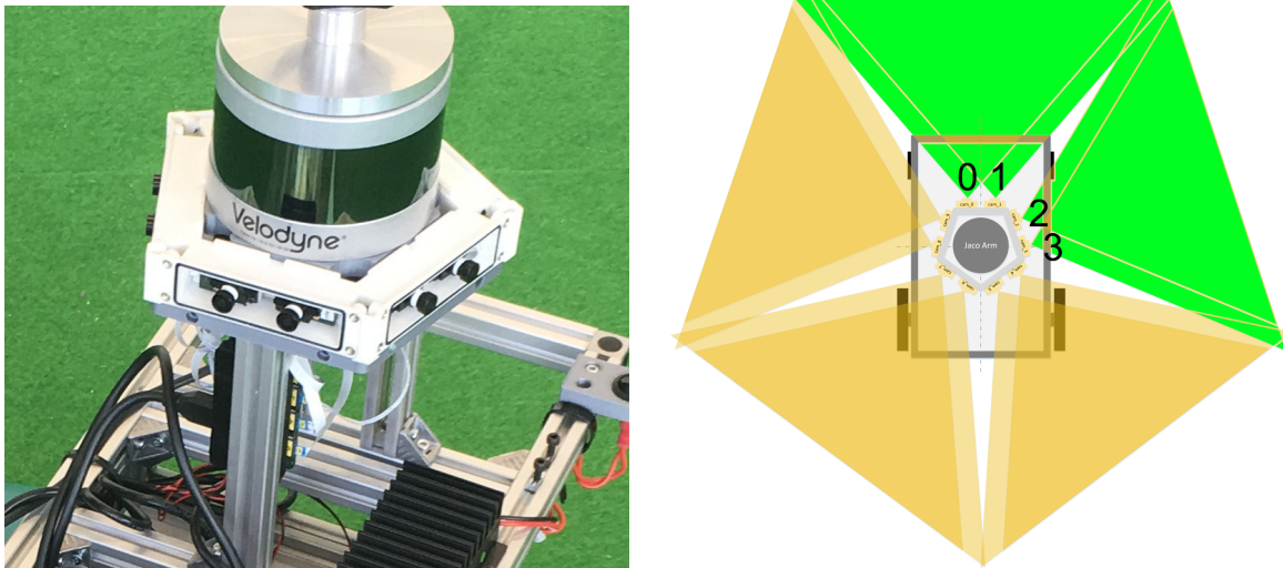
Figure 14: Trimbot Garden 2017 GT dataset [29]. Left : Pentagonal camera rig mounted on the robot with five stereo pairs. Right : Top view of camera rig with test set pairs (green field of view) and training set pairs (yellow field of view).
