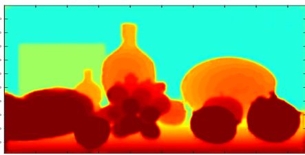
(i) Semi 2
