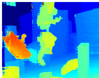
(c) PLSM [5]
