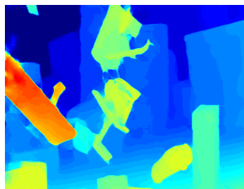
(i) semi 2
