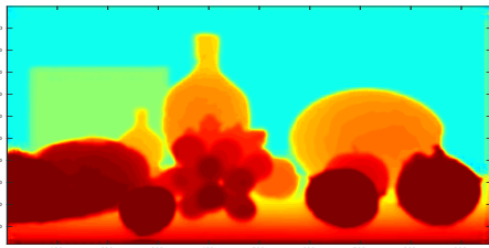
(g) Supervised 1
