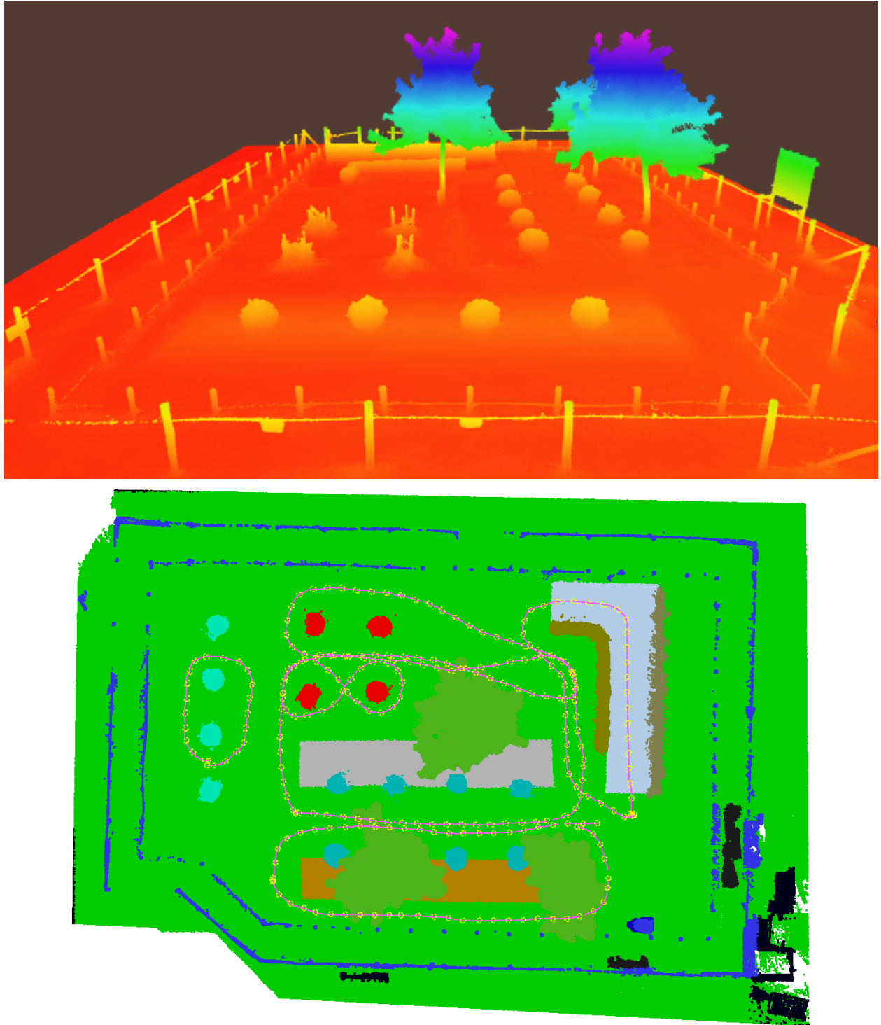
Figure 13: Trimbob Garden 2017 GT dataset [29]. Above : point cloud with color-encoded height. Below : semantic point cloud with trajectories (magenta line) and camera centers (yellow).
