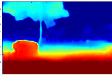
(g) Supervised 1
