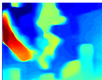
(e) Monodepth [7]
