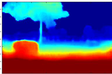
(i) Semi 2
