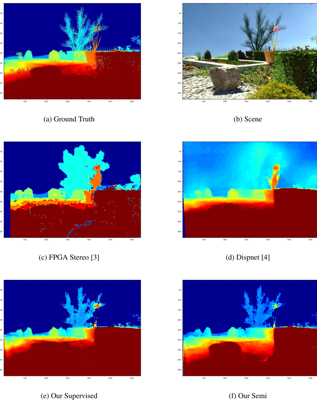
Figure 4: We fuse two initial raw disparity inputs (c)(d) to get a refined disparity map (e)(f) using our Supervised and Semi method on the synthetic garden dataset. (a) is the ground truth and (b) is the corresponding scene. Many, but not all, pixels from the fused result are closer to ground truth than the original inputs.
