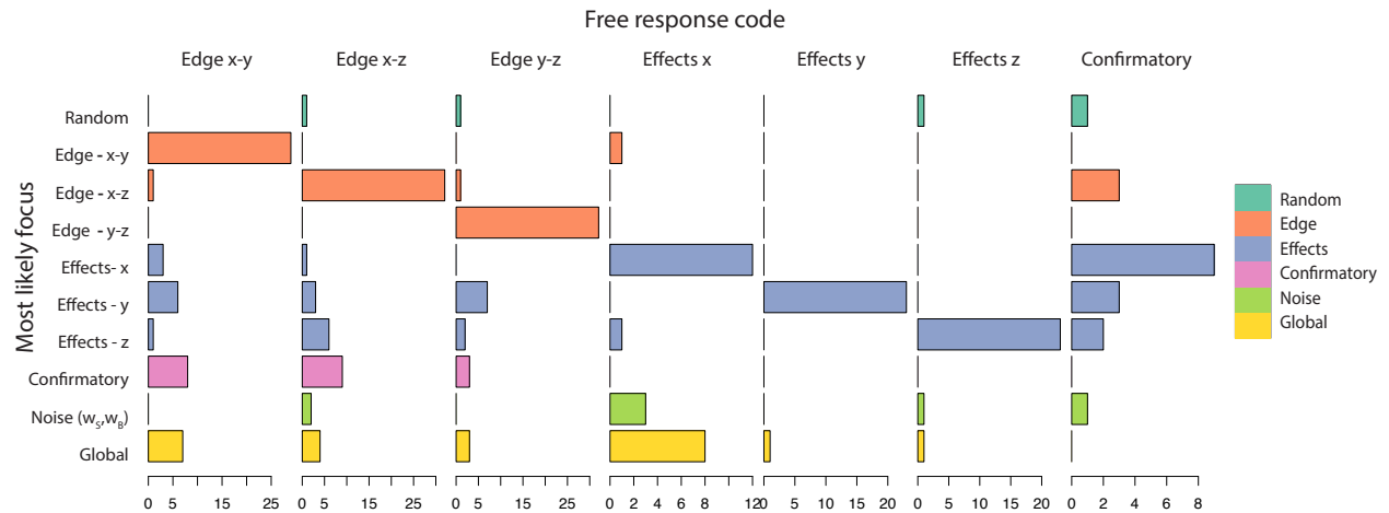
Figure 14: Model and free response code correspondence. Each plot is for trials assigned a particular free response code, each bar is for the number of trials for which that local focus was most likely given the intervention choice. Effect and edge coded queries were also diagnosed as such by the model fitting while confirmatory coded queries were most likely to be diagnosed as querying the effects of the root node(s) in the true model which always was (or included) x .
