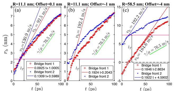
FIG. 5. Bridge growth corresponding to the cases presented in Fig. 4. Bridge location is measured from the line of approach. Bridge growth qualitatively changes beyond l_T . No line is fit in (b) to the ‘+’ markers within l_T , because there are not an appreciable number of data points. Note that the time here is measured from when a bridge appears in the equimolar plots; actual coalescence might have started before (see SM).
