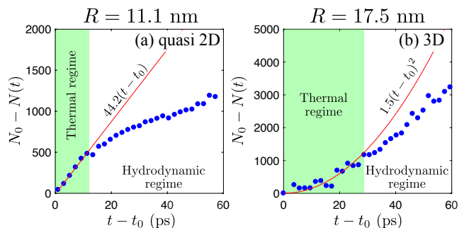
FIG. 6. The variation of the number of interface molecules, N(t) near a droplet front after the onset of coalescence at t_0 . (a) For quasi 2D droplets, N(t) is linear within the thermal regime. (b) For 3D droplets, N(t) \sim t^2 .
