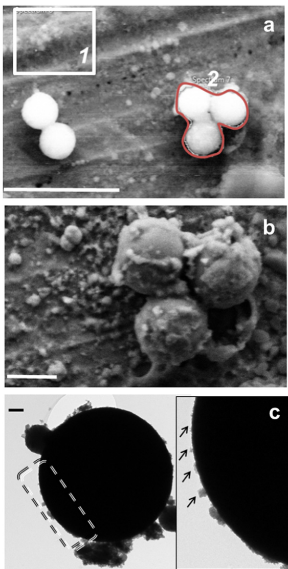
Fig. 3. a) SEM image of \text{Fe}_3\text{O}_4@Au particles, scale bar 5\ \mu\text{m} . b) HRSEM image of Au@Fe_3O_4 particles, scale bar 1\ \mu\text{m} . c) TEM image of \text{Fe}_3\text{O}_4@Au particles, scale bar 200\ \text{nm} , insert - magnified section shown in a check box of the microparticle surface.
