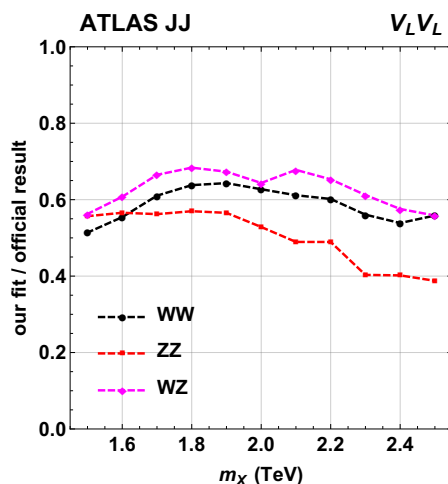
Figure 2. ATLAS hadronic search: ratio of observed exclusion limits obtained with this study to the ones of the official ATLAS result, as a function of the mass m_X of the exotic resonance for the WW (black), ZZ (red) and WZ (magenta) tagging selections.
