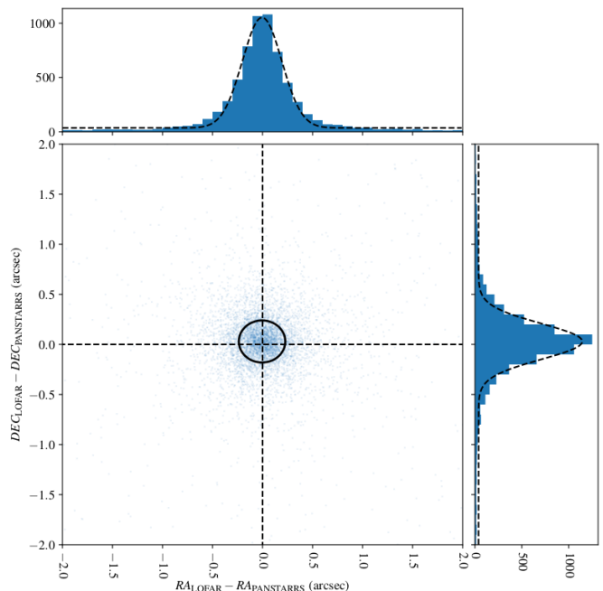
Fig. 8. Residual RA and Dec offsets for LOFAR detected sources matched with their Pan-STARRS counterparts. The histograms show the number of sources at various RA and Dec offsets and the ellipse shows the peak location (less than 0.02'' from the centre in both RA and Dec) and the FWHM ( \sigma \approx 0.2'' ) of the Gaussian functions that are fitted to the histograms of the offsets. Similar plots showing the same LoTSS-DR1 sources cross-matched with WISE or FIRST sources show comparable systematic offsets and standard deviations of less than 0.27'' and 0.3'' , respectively
