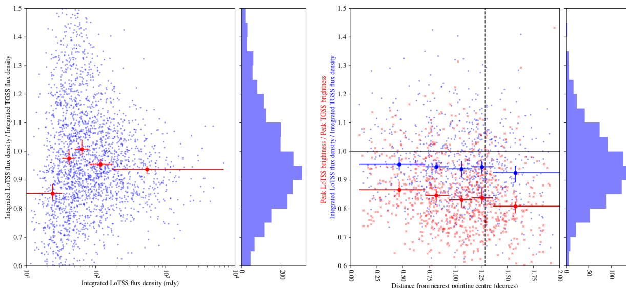
Fig. 9. LoTSS-DR1 to TGSS-ADR1 integrated flux density ratio as a function of integrated flux density (left) and for sources with an integrated flux density higher than 100 mJy as a function of distance from the nearest LoTSS pointing centre (right). Below 100 mJy the completeness of TGSS-ADR1 drops below 90% and, as a consequence, there is significant scatter in the integrated flux density ratio for sources below this limit. In the right panel we show that the 835 compact sources above this integrated flux density limit have a median integrated flux density ratio of 0.94 and a standard deviation of 0.14 (blue points) and a median peak brightness ratio of 0.83 and a standard deviation of 0.13 (red points). The thicker symbols show the median within bins indicated by horizontal error bars and the vertical error bars show the 95% confidence interval of the derived median value estimated by the bootstrap method. The bins are chosen to contain equal numbers of sources, which is 500 and 170 for the left and right panels respectively. The vertical dashed line shows the median distance between LoTSS pointings and many of the measurements at greater distance are due to the edges in the LoTSS-DR1 mosaic.
