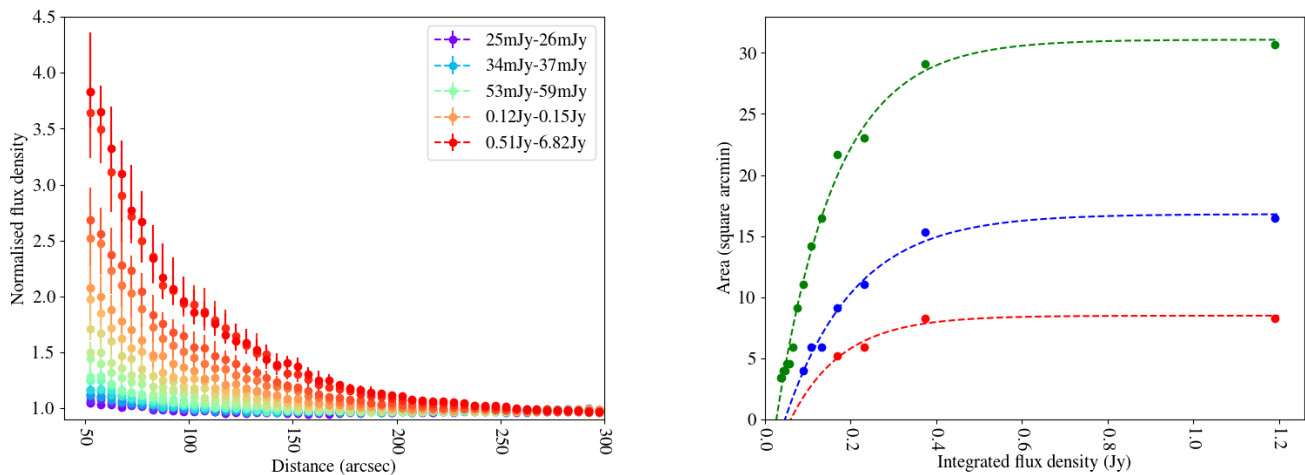
Fig. 11. Left: Profiles of the average standard deviation as a function of distance from compact LoTSS-DR1 sources in various integrated flux density bins. The integrated flux density bins were chosen to contain equal numbers of sources (110) and they vary from 25.0 mJy to 26.2 mJy (blue) to 510 mJy to 6820 mJy (red). The errors are 95% confidence intervals on the median values derived from the bootstrap method. Right: An estimate of the area in which the noise is 15% (green), 50% (blue), and 100% (red) higher than the thermal noise due to dynamic-range limitations around a bright source; the points show the measured values and the dotted lines show the best-fitting curves.
