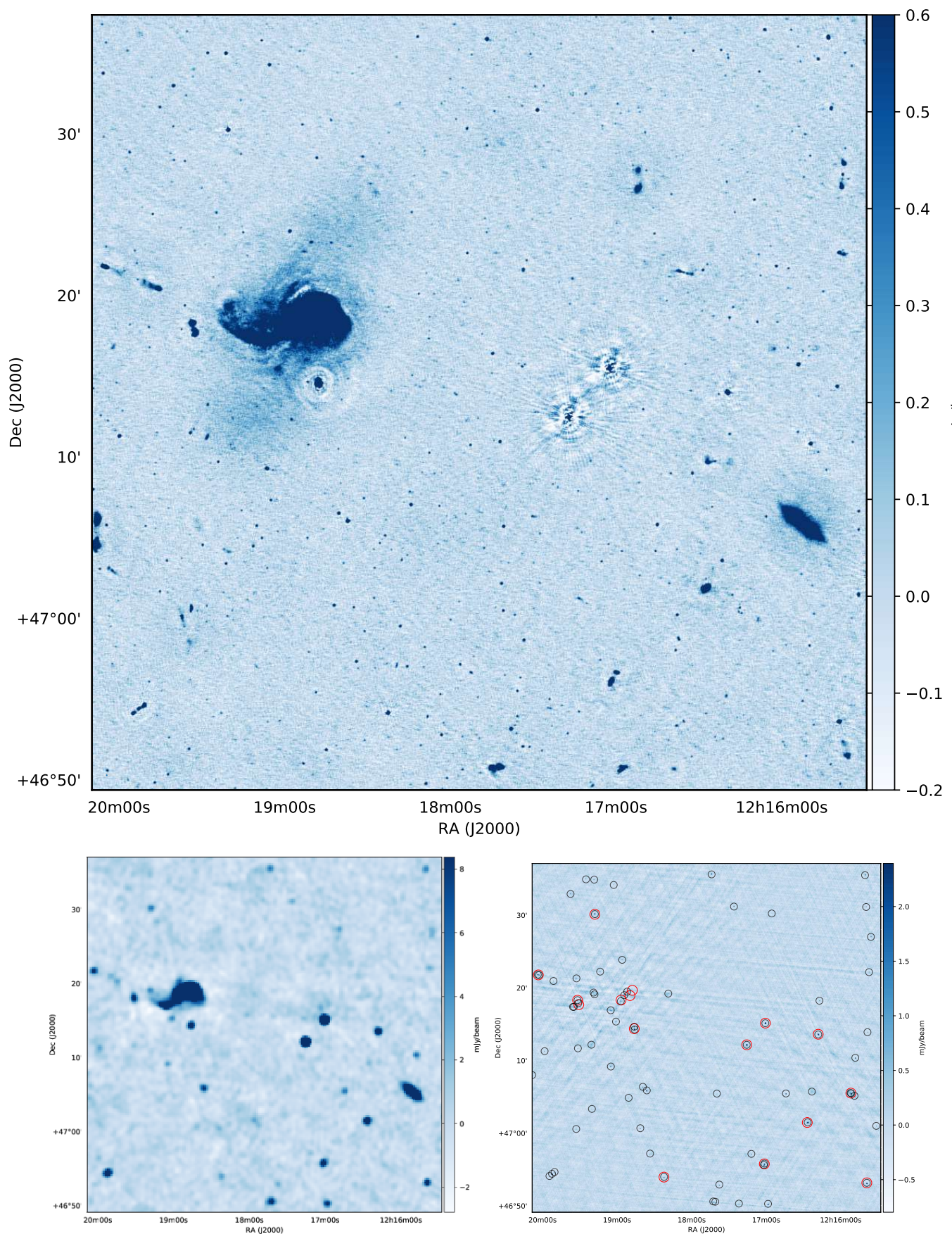
Fig. 4. Top figure shows an example of a LoTSS-DR1 image and bottom figures show the same region in NVSS (left) and FIRST (right). The black and red circles overlaid on the FIRST image show FIRST and TGSS-ADR1 sources, respectively. In this region there are 689 LoTSS-DR1 sources, 71 FIRST sources, 46 NVSS sources, and 16 TGSS-ADR1 sources. The resolution of the LoTSS-DR1 image is 6'' and the sensitivity in this region is approximately 70\mu\text{Jy beam}^{-1} . This field is dominated by the spectacular galaxy NGC 4258, which in the LoTSS-DR1 image has an extent of over 3000 synthesised beams, together with the smaller edge-on spiral galaxy NGC 4217.
