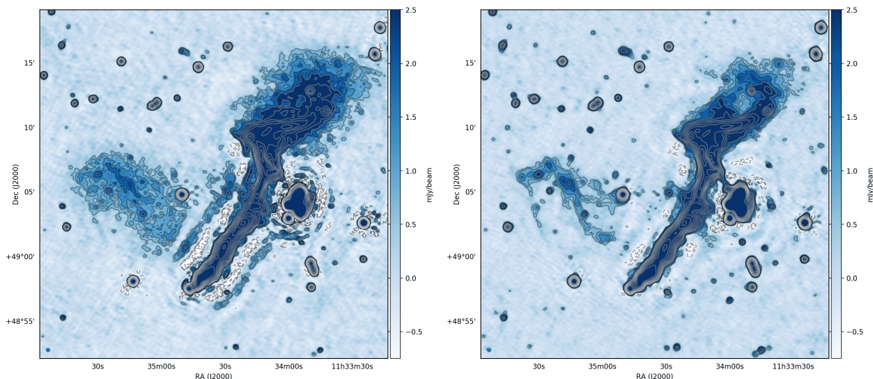
Fig. 15. Left panel shows the 20'' resolution LoTSS-DR1 mosaiced image of the galaxy cluster Abell 1314 and right panel shows an image produced from the same data but after improvements to the pipeline described in Sec. 5.1. The colour scale of the images are the same and the contours show the \pm\sqrt{1, 2, 4, \dots} \times 5\sigma levels where \sigma = 120\mu\text{Jy beam}^{-1} . The LoTSS-DR1 image of this cluster suffers from artificial haloes around the extended structures and a low dynamic range. The improved LoTSS image has a higher fidelity and is in good agreement with the independently processed image presented in Wilber et al. (2018b).
