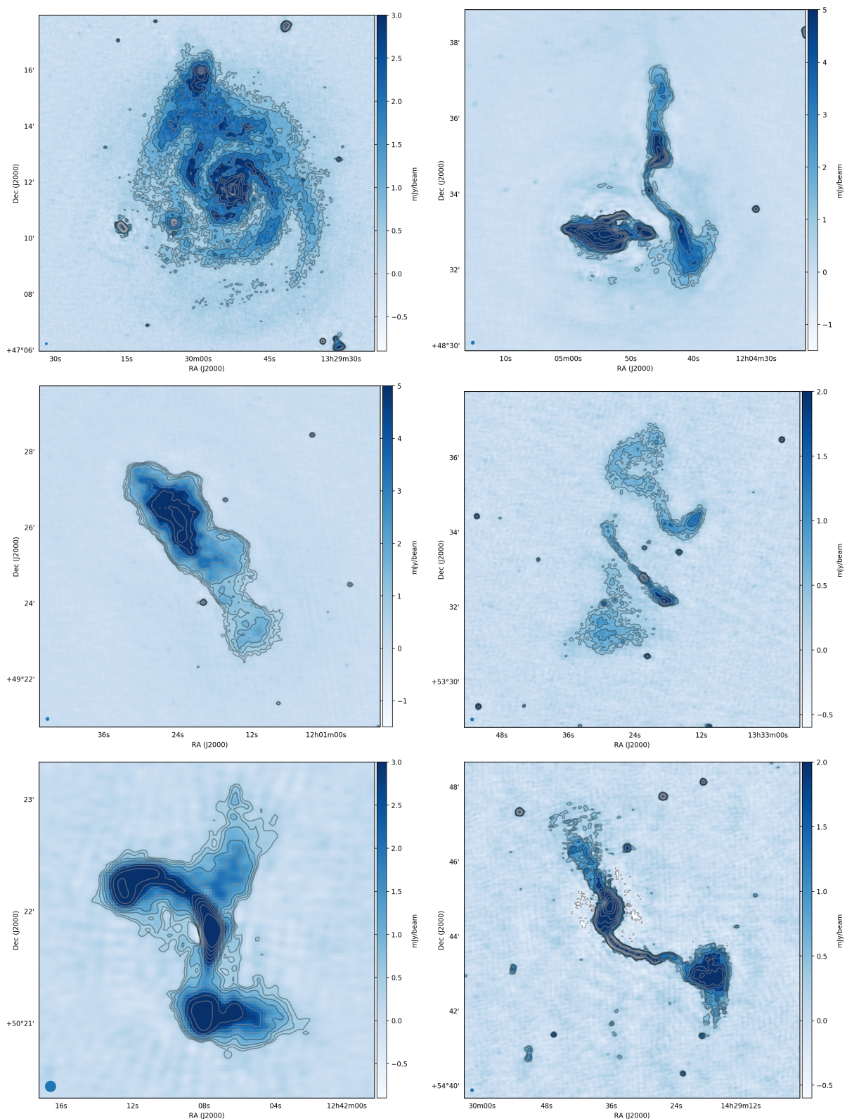
Fig. 6. Selection of resolved sources in the LoTSS-DR1 images with the colour scale and contours chosen for display purposes. The synthesised beam is shown in the bottom left corner of each image.
