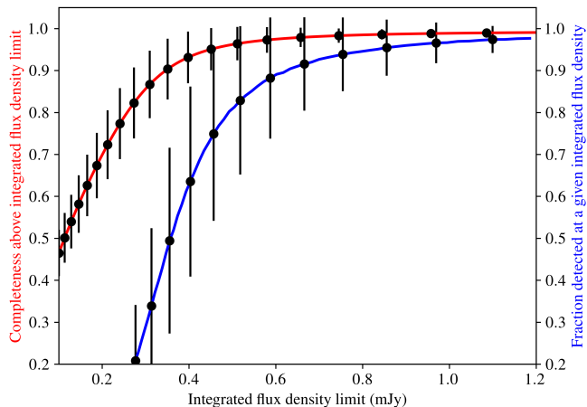
Fig. 14. Estimated point-source completeness of the LoTSS-DR1 catalogue. The red line shows the completeness above a given integrated flux density and the blue line shows the fraction of sources detected at a specific integrated flux density value. Because of the large number of sources injected during the simulation the Poisson errors are negligible but the errors bars reflect the standard deviation of the measurements as a function of position across the mosaic.
