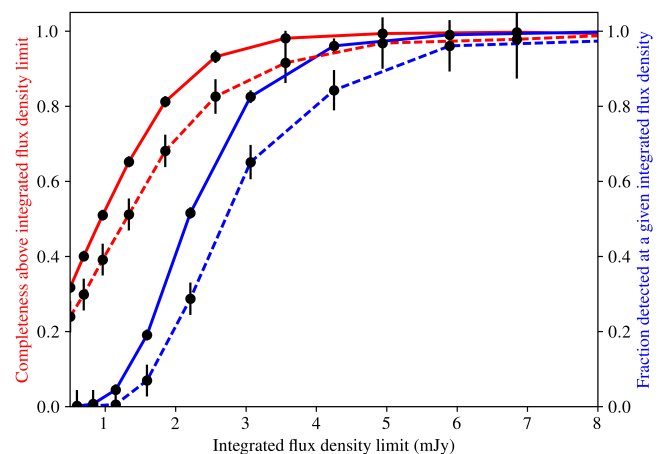
Fig. 13. Estimated point-source completeness for a 10 SB (1/24th of the data) for a single LoTSS-DR1 pointing. The red line shows the completeness above a given integrated flux density and the blue line shows the fraction of sources detected at a specific integrated flux density value. The solid lines show the results of the simulation in which point sources are injected into PyBDSF residual images and the dashed lines show results from when delta functions corrupted by realistic direction-dependent errors are injected into the uv -data before it is run through LoTSS-DR1. The error bars give the Poisson errors.
