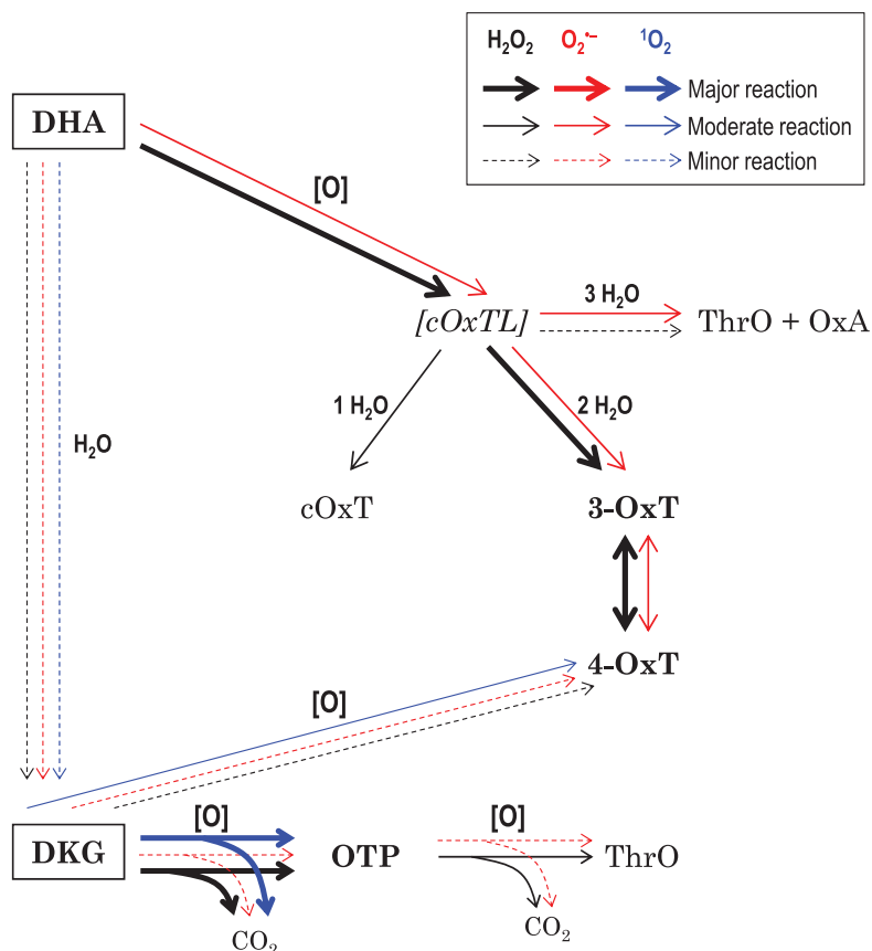
Figure 3. Deduced pathways of dehydroascorbic acid and diketogulonate degradation in the presence of H 2 O 2 , superoxide, or singlet oxygen.
