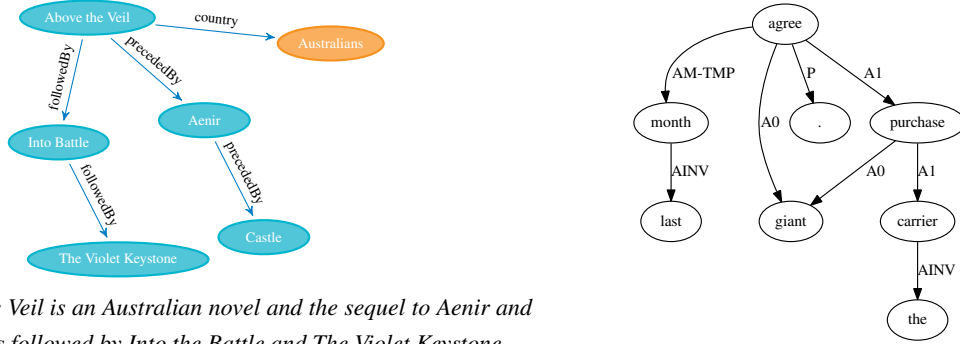
Figure 1: Source RDF graph - target description (a). Source dependency graph - target sentence (b).
