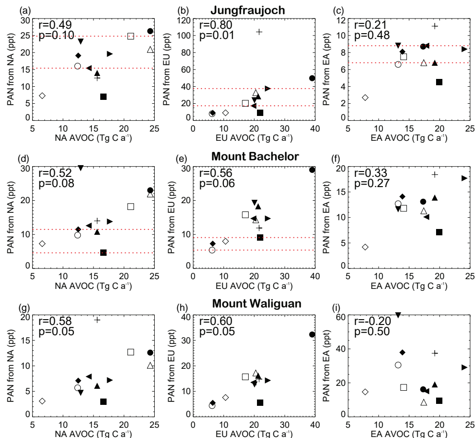
Figure 5. SRRs diagnosed as the difference between the SRI and SR6xx simulations in Table 1 for PAN (ppt) at Jungfrauoch (a, b, c), Mount Bachelor (d, e, f), and Mount Waliguan (g, h, i) in each HTAP1 model (see Table 1 for the symbol assigned to each model) versus the annual emission of anthropogenic VOCs (AVOCs; \text{Tg C a}^{-1} ) within the NA (a, d, g), EU (b, e, h), and EA (c, f, i) source regions. The Spearman's rank correlation coefficient (more robust to outliers than the traditional Pearson coefficient) and associated p value are shown in each panel. The horizontal red lines correspond to the values identified with the red symbols in Fig. 4.
