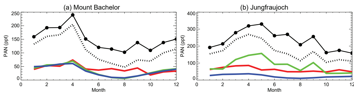
Figure 1. Multi-model monthly mean total PAN mixing ratios (black circles and solid lines) at Mount Bachelor (a) and Jungfrauoch (b). We take the difference between the base simulation (SR1) and one in which emissions are decreased by 20 % and then multiply the difference by 5 to estimate a 100 % contribution associated with anthropogenic precursor emissions from Europe (green), North America (red), and East Asia (blue). The sum of the anthropogenic contribution from these three regions is shown (dashed black) for comparison with total simulated PAN.
