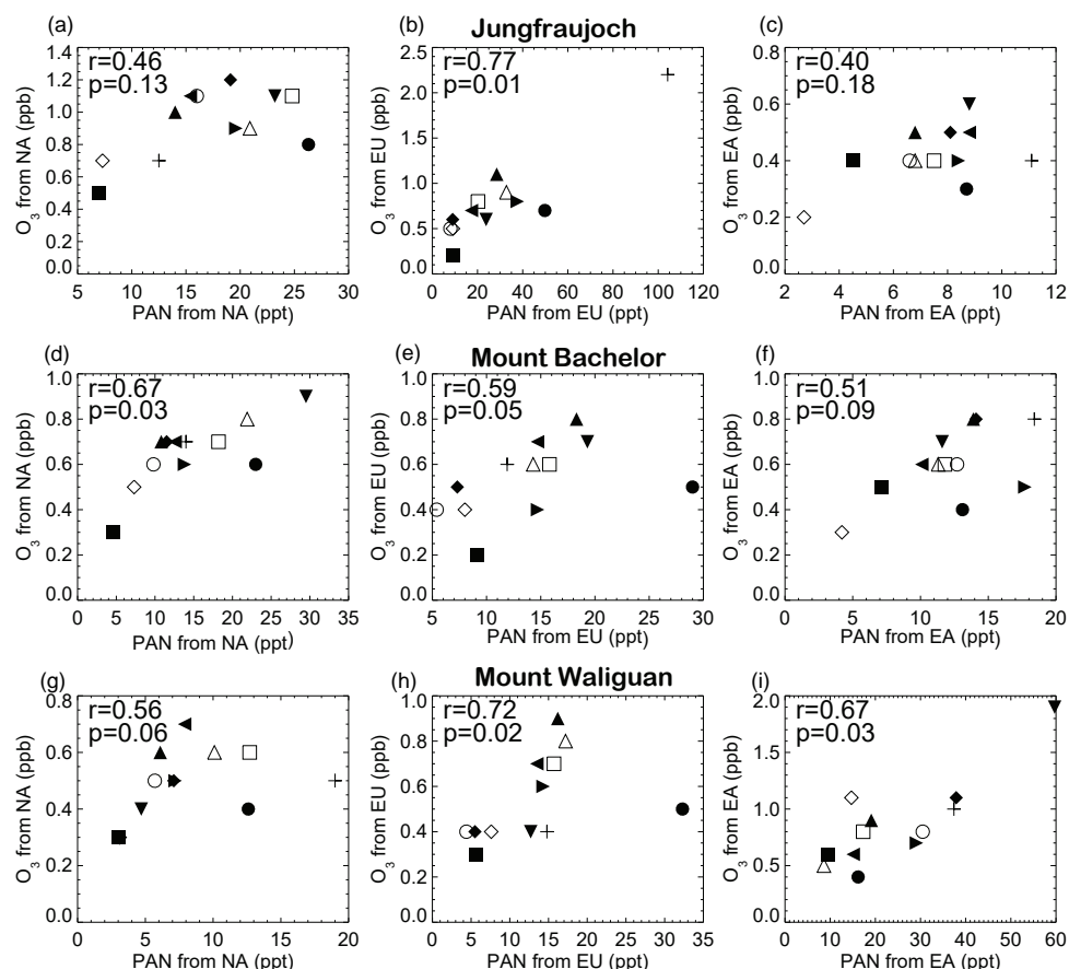
Figure 7. SRRs for O 3 versus PAN at Jungfrauoch (a, b, c), Mount Bachelor (d, e, f), and Mount Waliguan (g, h, i), obtained by subtracting the SR6XX from the SR1 simulations (Table 2) available from 12 models, for which XX denotes the NA (a, d, g), EU (b, e, h), or EA (c, f, i) source region. Each model thus contributes one point (symbols defined in Table 1) in each panel. Spearman's (rank) correlation coefficient and p values are also shown.
