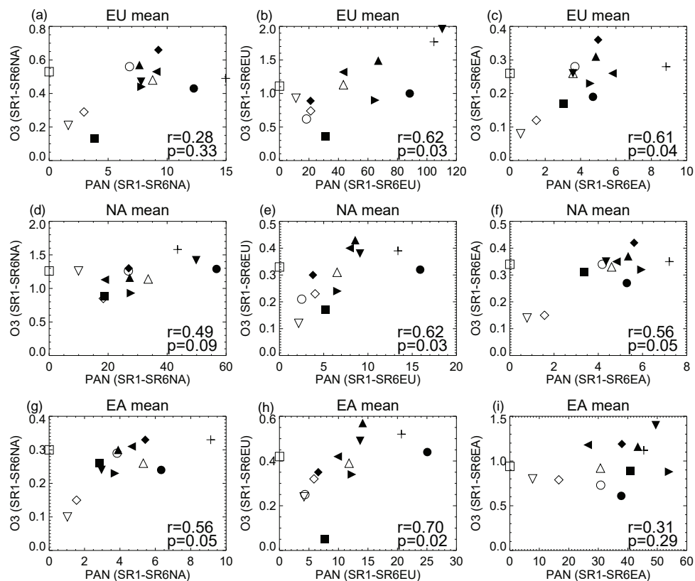
Figure 8. SRRs for O_3 versus PAN in surface air over each of the HTAP1 northern midlatitude continental regions: EU (a, b, c), NA (d, e, f), and EA (g, h, i), obtained by subtracting the SR6XX from the SR1 simulations, for which XX denotes the NA (a, d, g), EU (b, e, h), or EA (c, f, i) source region. Spearman's (rank) correlation coefficient and p values are also shown. Symbols denote individual models as defined in Table 1. STOC-HadAM3-v01 is excluded here as an outlier that artificially raised the correlation significance.
