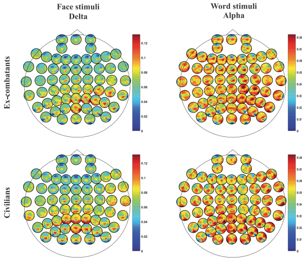
FIGURE 4. Absolute value of the imaginary part of coherency. These maps correspond to the face stimuli in the delta band, and to the word stimuli in the alpha band, as they were further validated to be the top-ranked discriminative features.
