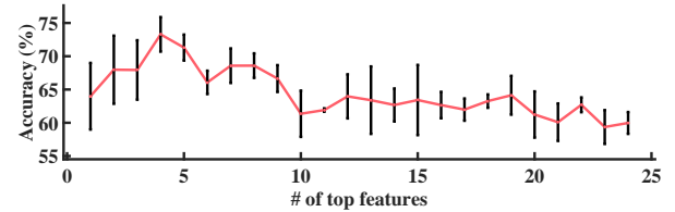
FIGURE 5. SVM-RFE results on FCN features. Average classification accuracy of the top-ranked features. The error bars represent the standard deviations.
