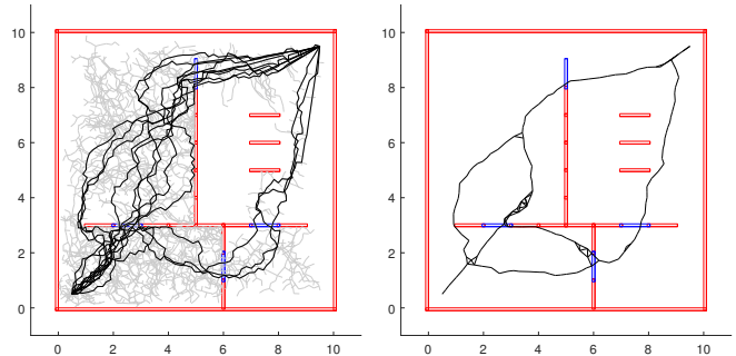
(a) Input trajectories. Grey lines show the full RRTs, and black lines the solution paths. (b) Embedded Reeb graph. Note show the full RRTs, and black lines the representation of distinct trajectory classes.
