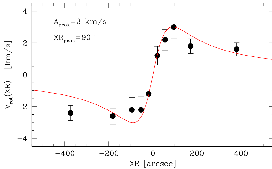
Figure 11. Rotation curve of M5. The black circles mark the stellar mean velocity as a function of the projected distance on either side of the rotation axis (XR) for the intervals listed in Table 4. The red line, which well reproduces the observed curve, has the functional form expressed in Equation (1), with A_{\text{peak}} = 3 \text{ km s}^{-1} and \text{XR}_{\text{peak}} = 90'' .
