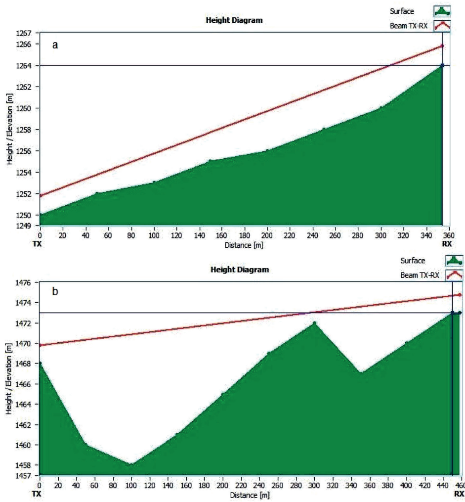
Figure 2 Path length beam and underlying surface topography between the LAS transmitter (TX) and receiver (RX) at (a) Somerton and (b) Truro farms
