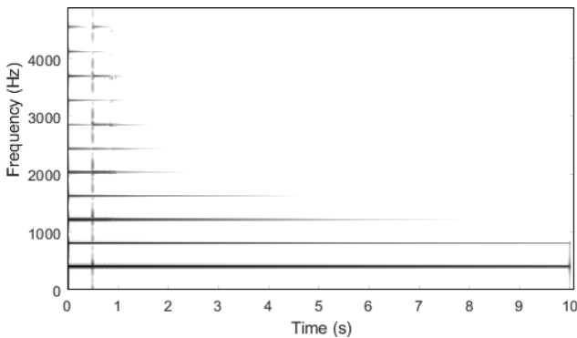
Figure 12: Spectrogram of a plucked stiff string colliding with a point rigid barrier at (x = L/2; y = 0.99 * U(t_0 = 0.5s)) , from t = 0.5s , for K_c = 5 * 10^8 N.m^{-\alpha} , and \alpha = 1.6 .
