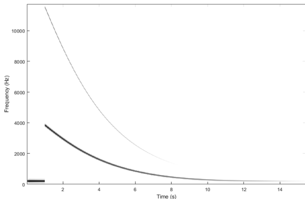
Figure 2: Spectrogram of u for the single-degree-of-freedom system with a cubic spring term activated at t = 1s with \omega_1 = 300m^{-1/2}.s^{-1/2} , initial conditions u^0 = 1m , u^1 = 1m .
