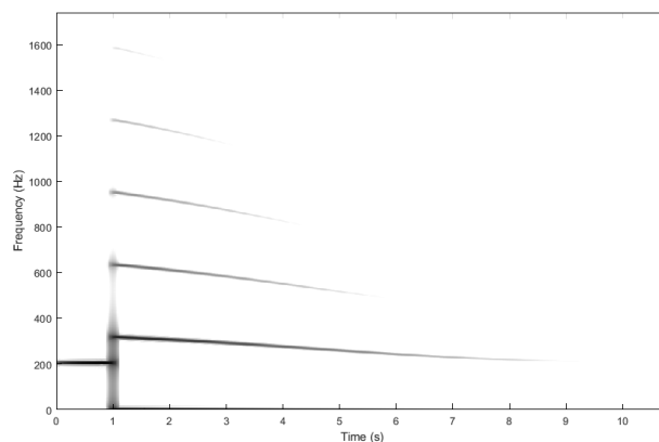
Figure 4: Spectrogram of u for the single-degree-of-freedom system with a stiff unilateral non-linear spring appearing at t_0 = 1s . K_c/M = 1.6 * 10^{10}m^{-1/2}.s^{-1/2} , \alpha = 1.9 initial conditions u^0 = 1m , u^1 = 1m .
