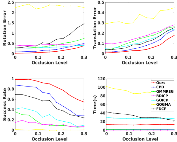
Figure 6: Occlusion Experiment
