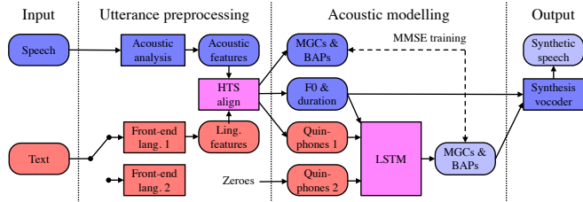
Fig. 1. Overview of bilingual cyborg speech synthesis system.
