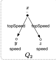
Fig. 1: Graph patterns
