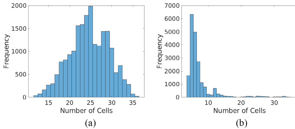
Figure 9. Histograms showing the posterior distributions on the number of Voronoi cells used to partition the spatial domain for (a) the case where straight rays between transmitters and receivers are used to calculate the first times of arrival and (b) where the MSFM has been used to consider the effects of raybending on the first times of arrival.
