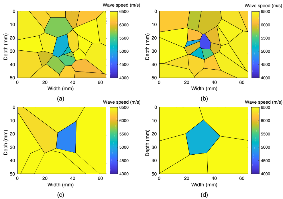
Figure 8. Samples from the posterior distribution of Voronoi diagrams. Plots (a) and (b) are the 2000th and 20 000th samples respectively arising from the case where straight rays are used in the forward model. Plots (c) and (d) are the 2000th and 20 000th samples arising from the case where the effects of raybending are included in the forward model.
