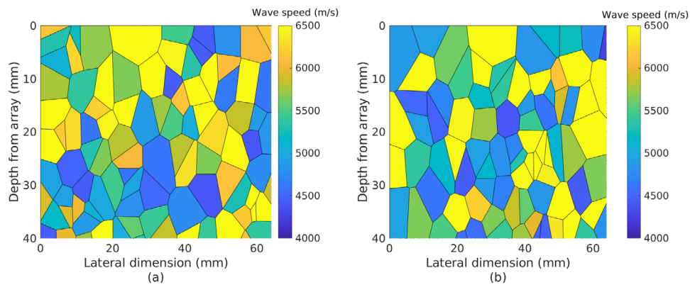
Figure 11. Voronoi tessellations drawn from the posterior distribution for the reconstruction of a random media from through-transmission data. Plot (a) shows iteration 35 000 and plot (b) shows iteration 100 000.
