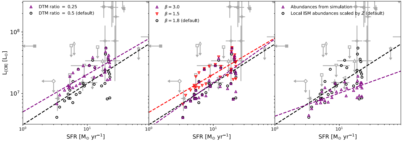
Figure 11. Result of deviating from the default assumptions of \hat{\text{S}}\hat{\text{I}}\hat{\text{G}}\hat{\text{A}}\hat{\text{M}}\hat{\text{E}} . Purple triangles show the simulated galaxies in the L_{\text{C II}}\text{--SFR} diagram after reducing the DTM ratio by a factor of 2 (left), changing the GMC mass spectrum to one that is more bottom heavy or top heavy (middle), and adopting abundances that better match the cosmological simulation (right). Black circles show the location of model galaxies with the default assumptions of \hat{\text{S}}\hat{\text{I}}\hat{\text{G}}\hat{\text{A}}\hat{\text{M}}\hat{\text{E}} . Observations are shown with gray symbols as in Figure 6.
