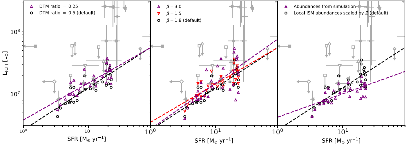
Figure 11. Result of deviating from the default assumptions of SÍGAME. Purple triangles show the simulated galaxies in the L_{\text{CII}} -SFR diagram after reducing the DTM ratio by a factor of 2 (left); changing the GMC mass spectrum to one that is more bottom- or top-heavy (middle); adopting abundances that better match the cosmological simulation (right). Black circles show the location of model galaxies with the default assumptions of SÍGAME. Observations are shown with gray symbols, as in Figure 6.
