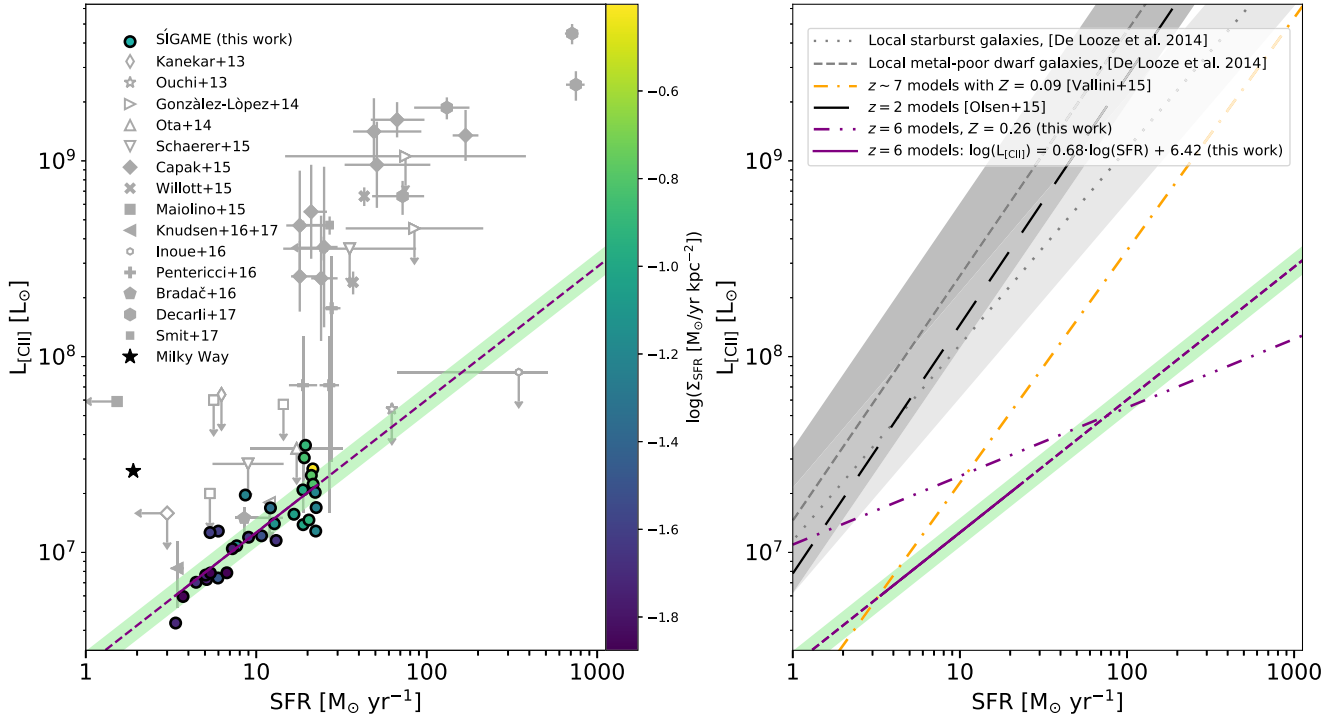
Figure 6. Left: the [C II] luminosity vs. SFR. For the sake of clarity, we have not included MS0451-H ( z = 6.703 ) in the plot. This source has L_{[\text{C II}]} < 3 \times 10^5 L_{\odot} and \text{SFR} \sim 0.4 M_{\odot} \text{ yr}^{-1} (Knudsen et al. 2017) and lies about 1 dex below our fitted relation. All SFRs have been converted to a Chabrier IMF where applicable. Right: a comparison with other, observed and simulated, [C II]–SFR relations. Shown are the [C II]–SFR relations derived by De Looze et al. (2014) for local metal-poor dwarf galaxies (gray dashed line) and local starburst galaxies (gray dotted line); gray dashed and dotted lines, respectively, with the shaded regions indicating the rms scatter of these relations). Also shown are simulated relations of z = 2 main-sequence galaxies (black long dashed line; Olsen et al. 2015) and z \sim 7 galaxies (orange dashed-dotted line; Vallini et al. 2015).
