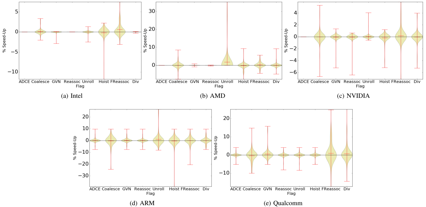
Fig. 9. Percentage speed-up from individual flags for each platform
