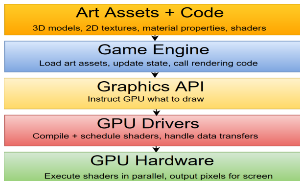
Fig. 1. Graphics Stack
