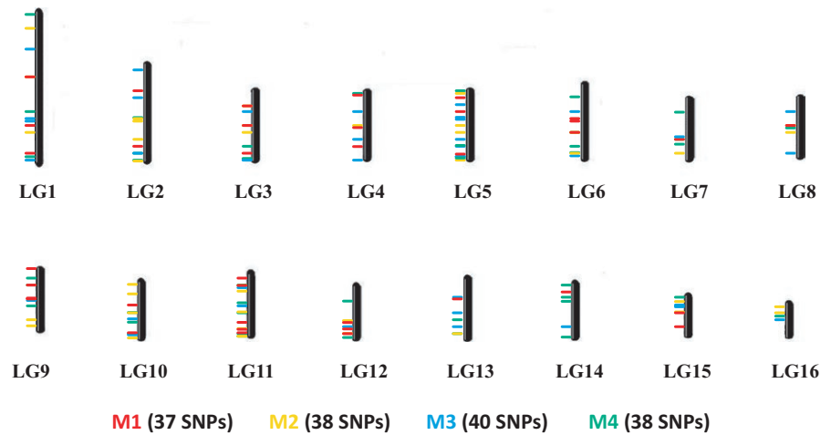
FIGURE 3 Chromosome map showing the SNP positions of the four reduced assays (M1–M4)
