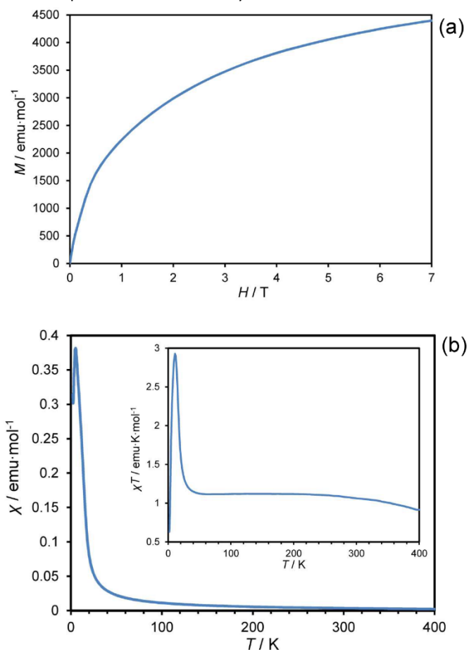
Figure 2: (a) Magnetisation against magnetic field curve of [Ni(qs) 2 ] measured at 2.0 K. (b) Magnetic Susceptibility of [Ni(qs) 2 ] at varying temperature measured in a field of 1000 Oe and (inset) Temperature dependence of \chi T for [Ni(qs) 2 ] measured at 1000 Oe.
