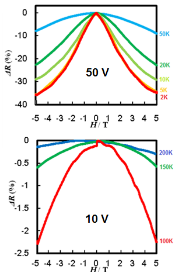
Figure 4: Magnetic field dependence of resistance of [\text{Ni}(\text{qs})_2] at various temperatures.
