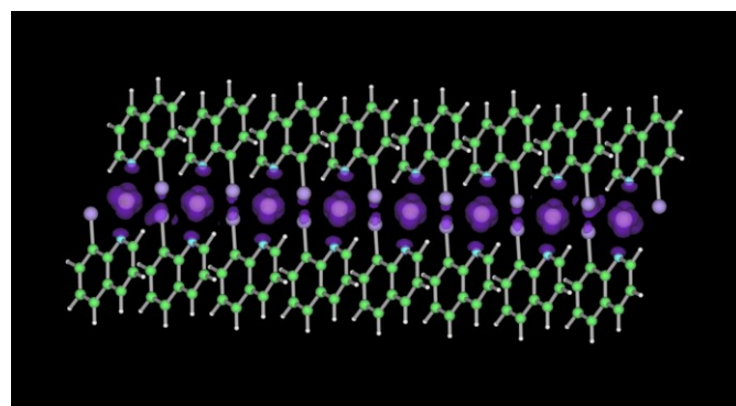
Figure 6: Calculated spin density of an 8-mer chain of [\text{Ni}(\text{qs})_2] .
