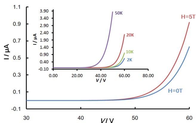
Figure 3: Magnetic field dependence of I-V at 2 K for [\text{Ni}(\text{qs})_2] , the inset shows the non-linear I-V behaviour for the same device.
