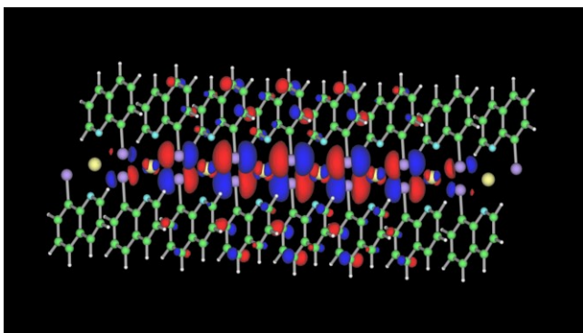
Figure 5: Calculated HOMO of an 8-mer chain of [\text{Ni}(\text{qs})_2] .
