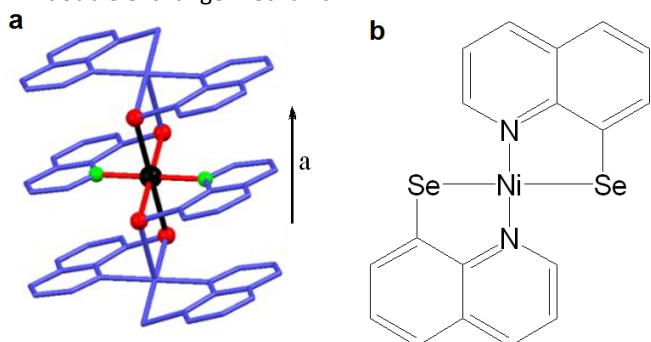
Figure 1: (a) Structure of [Ni(qt) 2 ] and (b) new analogue [Ni(qs) 2 ] substituting sulfur for selenium.
