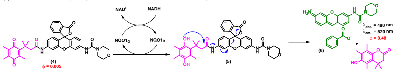
(C) Different probes and their respective reporters described by McCarley group:
