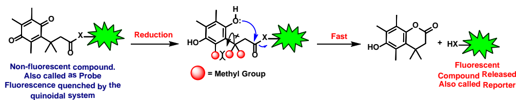
(B) Reductive activation via enzymatic processes involving NQO1 for releasing the fluorescent probe:
