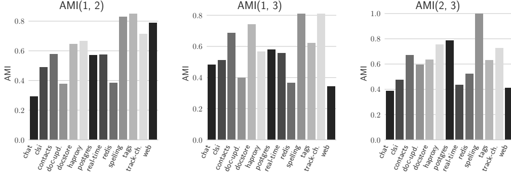
Figure 3. Pairwise adjusted mutual information (AMI) scores between 3 measurements.
