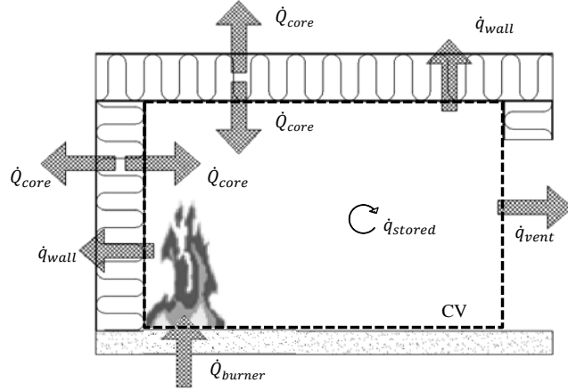
Fig. 3: Schematic of the Control Volume and the energy balance within the CV. Not to scale.
