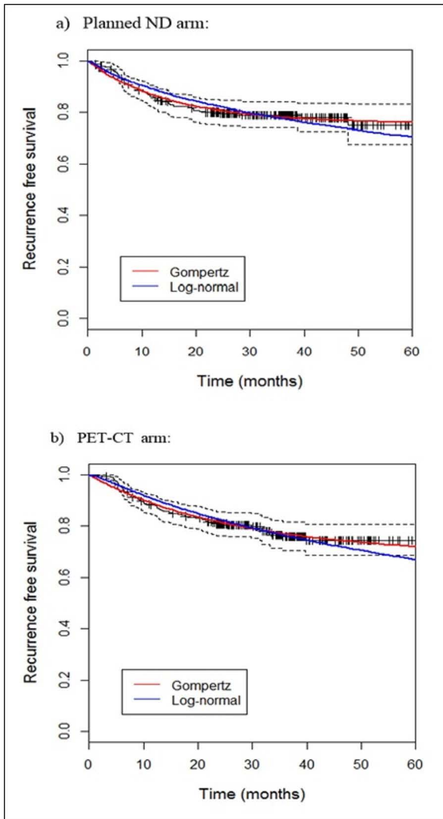
Figure S2. Plot of parametric survival curves (using Gompertz and Log-normal model specifications) against PET-Neck trial data on patient recurrence free survival
