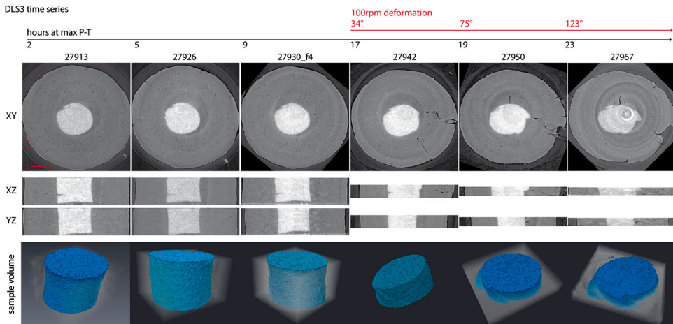
Figure 15. Textural changes in sample DLS3, shown by orthogonal slices through tomographic reconstructions, and the segmented central Fe–S-bearing region to show changes in 3-D shape. Orthogonal slices are zoomed into the central sample portion (field of view: 3 mm \times 3 mm): white: Fe–S+olivine, grey:forsterite capsule, dark grey: graphite furnace surrounded by gasket. Scans obtained as a time series, left to right, during annealing at high-P, T after 2, 5 and 9 h, respectively, and then after torsional deformation corresponding to a total differential anvil rotation of 34°, 75° and 123°, as described in the main text.
