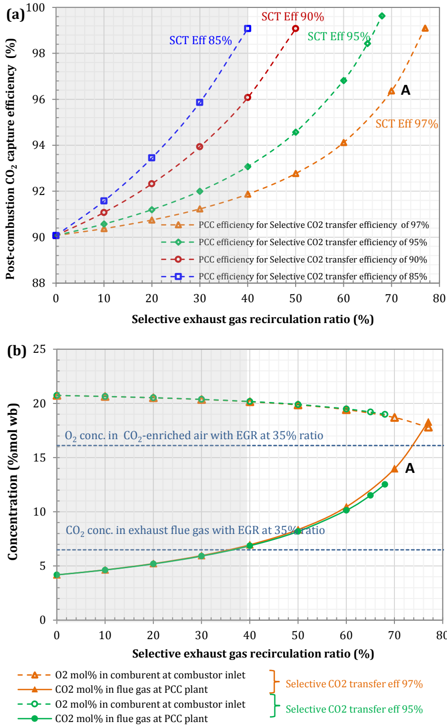
Figure 4.- (a) Sensitivity of the post-combustion CO 2 capture efficiency and (b) Sensitivity of CO 2 concentration in the flue gas at the inlet of the post-combustion capture system and O 2 concentration in the CO 2 -enriched combustion air to the selective exhaust gas recirculation ratio, for a range of selective CO 2 transfer (SCT) efficiencies. SEGR in parallel for 90% overall CO 2 capture level.
