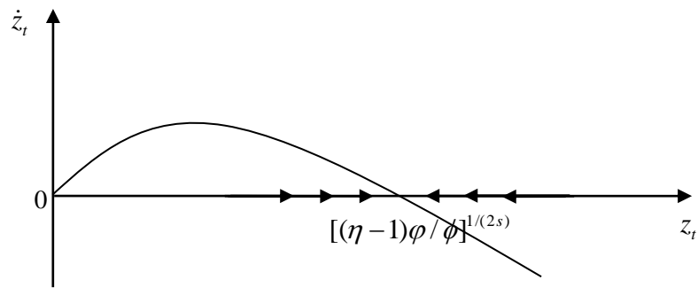
Figure 1: Phase diagram
