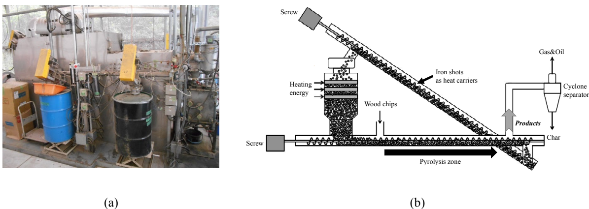
FIGURE 1. Developed fast pyrolysis reactor with Auger-type modules (a) overview and (b) schismatic flow system.
