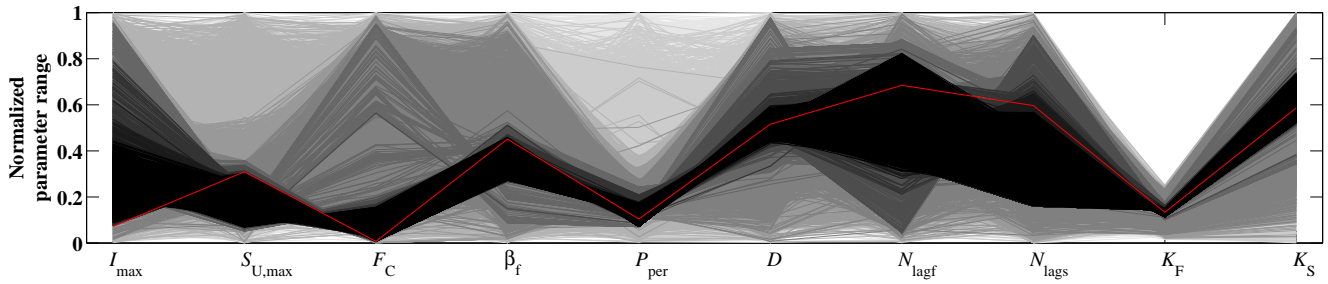
Figure 5. Normalized parameter plot for FLEXA. Darker colors indicate parameter sets that satisfy larger numbers of process constraints. The red trajectory indicates \theta_{\text{best}} .
