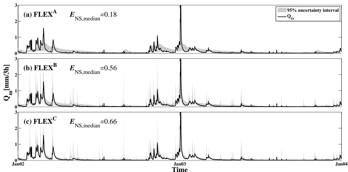
Figure 1. The observed hydrograph and the 95 % uncertainty interval of the modeled hydrograph derived from the complete set of constrained but un-calibrated parameter sets for the three different model set-ups (a) FLEX A , (b) FLEX B and (c) FLEX C for the 2 years (2002–2003) of calibration period. The median performance of the constrained but un-calibrated models based on Nash–Sutcliffe efficiency ( E_{NS,median} ) are reported (Gharari et al., 2014).
