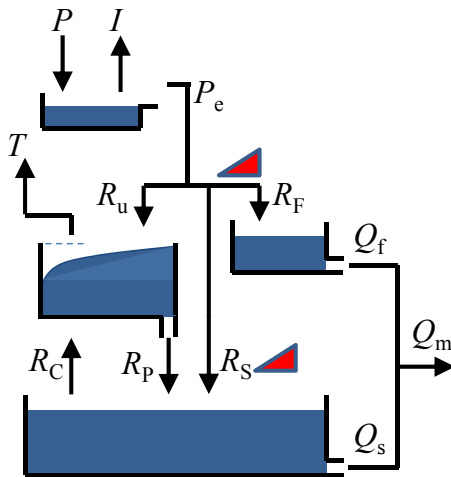
Figure 4. The model structure of FLEXA. Precipitation is indicated by P ; I and T represent components of evaporation which are interception and transpiration respectively. Q_f and Q_s indicate the fast and slow components that make the total model output ( Q_m ). The water balance equations and constitutive functions are presented in the companion paper (Gharari et al., 2014).
