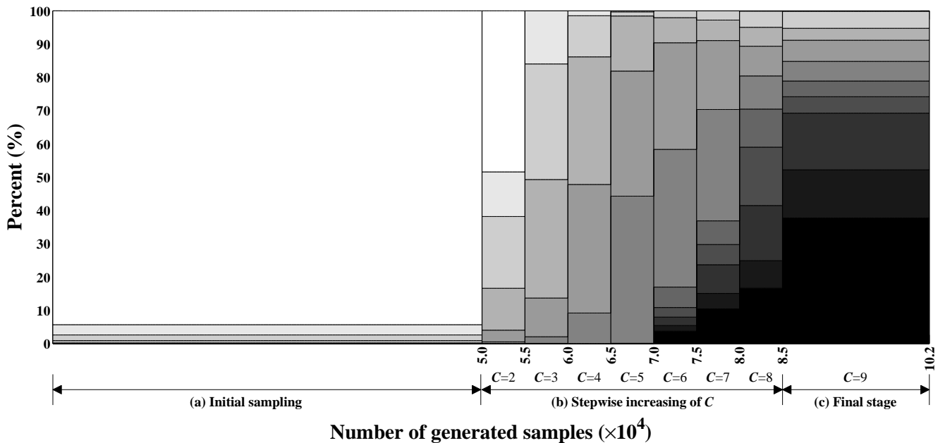
Figure 7. Percentages of samples generated at each stage that satisfy a given number of process constraints. White indicates no satisfied constraints, and progressively darker colors indicate increasing numbers of satisfied constraints. (a) The initial sampling ( N = 50\,000 ). (b) Stepwise increase of C , thus requiring an increasing number of process constraints to be satisfied at each stage, and (c) the final stage of the search when C is set to the maximum number of design constraints (here 9), at which point the search continues until 8000 behavioral parameter sets have been located.
