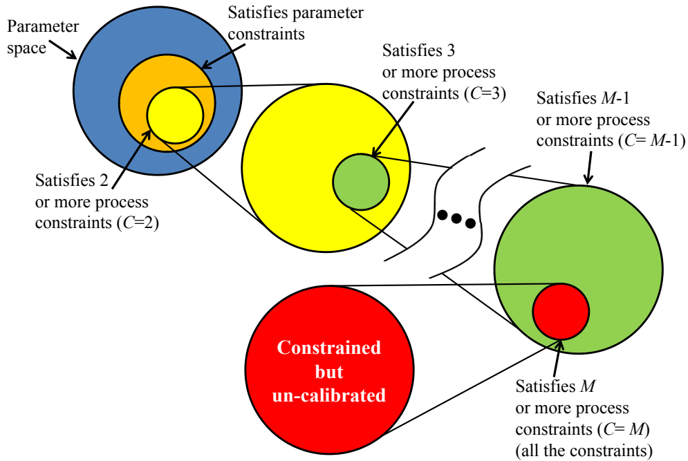
Figure 3. A conceptual illustration of stepwise search for the parameter space satisfying all of the parameter and process constraints.
