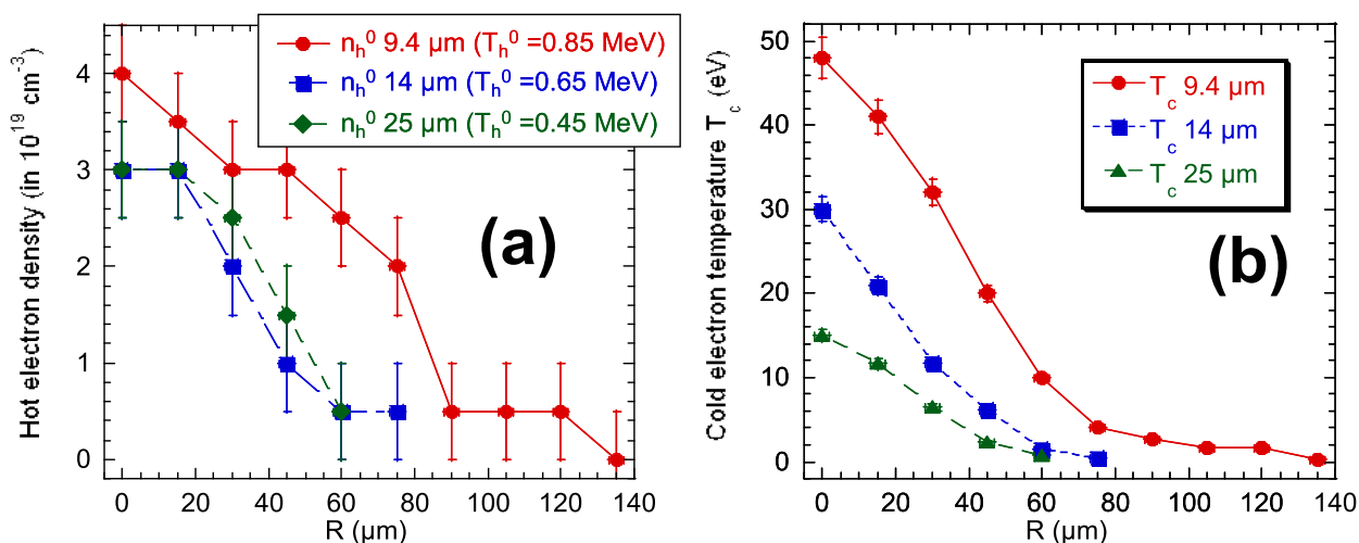
FIG. 4. (a) Spatial profile of the hot electron density for three Al target thicknesses at fixed laser intensity \sim 5 \times 10^{19} \text{ W/cm}^2 and pulse duration \tau = 320 \text{ fs} . The average hot electron temperature T_h^0 is also indicated and is found to agree with the scalings suggested by Ref. 27 for similar target thicknesses ( \sim 10 \mu\text{m} ). (b) Corresponding profiles of the bulk electron temperature.
