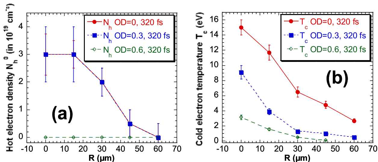
FIG. 3. (a) Spatial profile of the hot electron density for a 25 \mu\text{m} thick Al target irradiated with pulse duration \tau = 320 \text{ fs} at I \sim 5 \times 10^{19} \text{ W/cm}^2 (dots), I \sim 2.5 \times 10^{19} \text{ W/cm}^2 (squares), and I \sim 1.2 \times 10^{19} \text{ W/cm}^2 (diamonds). (b) Corresponding profiles of the bulk electron temperature. The inferred average hot electron temperature is T_h^0 = 0.45 \text{ MeV} in the first two cases.
