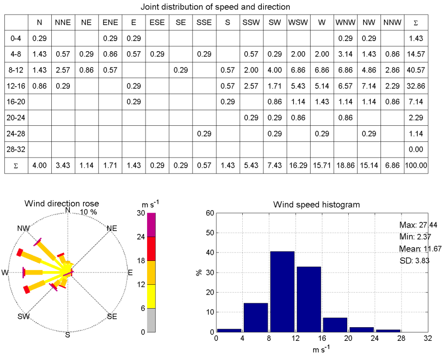
Figure 6. For the 340 cases where there was a wind increase above warm-core eddies and a decrease downstream: distribution in % and m s^{-1} of wind speed and direction (top); wind direction rose (bottom left) and wind speed histogram (bottom right) at the entrance of the eddy upstream.
