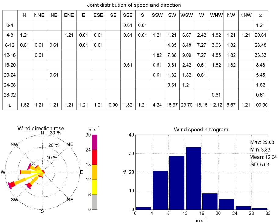
Figure 7. For the 180 cases where there was no wind increase above warm-core eddies: distribution in % of wind speed and direction and m s^{-1} (top); wind direction rose (bottom left) and wind speed histogram (bottom right) at the entrance of the eddy upstream.
