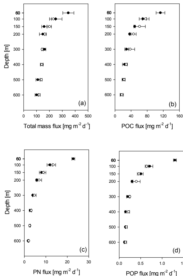
Figure 2. Fluxes of (a) total mass and (b) particulate organic carbon (POC), (c) particulate nitrogen (PN) and (d) particulate organic phosphorus (POP) during the deployment of two STDT in the ETNA. Solid symbols are used for deployment no. 1 and open symbols for deployment no. 2.
