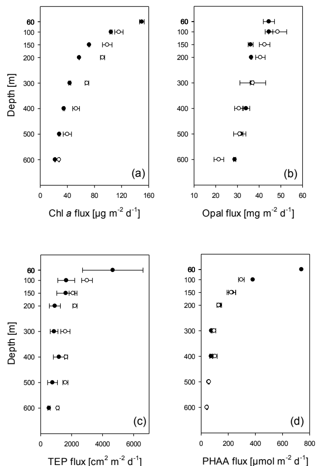
Figure 3. Fluxes of (a) chlorophyll a (Chl a ), (b) opal, (c) TEP and (d) PHAA during the deployment of two STDT in the ETNA. Solid symbols are used for deployment no. 1 and open symbols for deployment no. 2.
