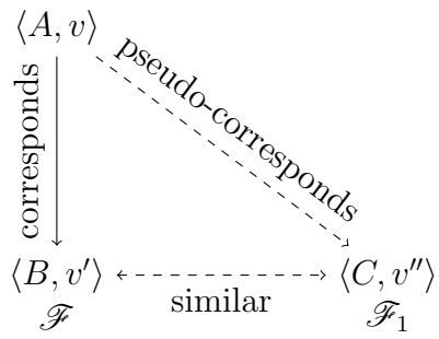
Figure 1: Corollary 1
