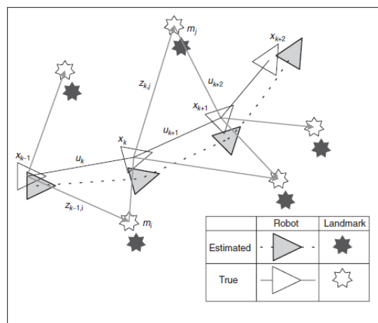
Figure 1. The essential SLAM problem.
