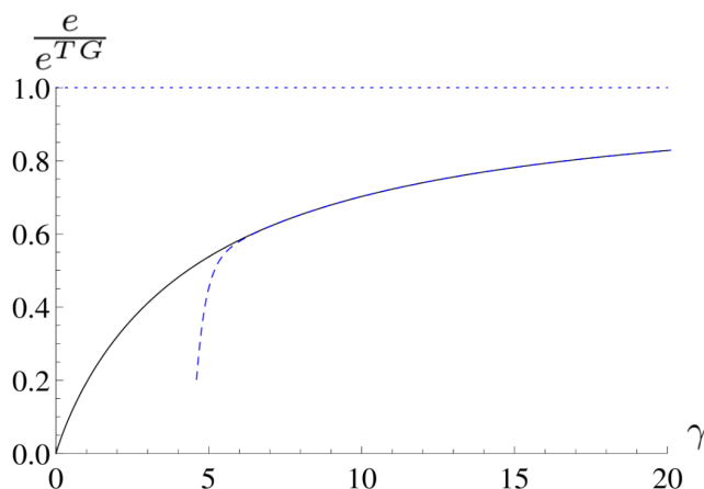
Figure 15: Ground state energy per particle e in units of its value in the Tonks-Girardeau limit e^{TG} , as a function of the dimensionless interaction strength \gamma . Numerically exact result (black), compared to 20 th -order expansion in the strongly-interacting regime (blue, dashed) as given by Eq. (104). The value in the Tonks-Girardeau limit (horizontal, blue, dotted) is also indicated on the figure.
