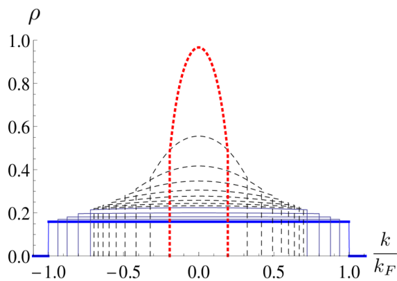
Figure 2: Dimensionless density of pseudo-momenta \rho as a function of dimensionless pseudo-momentum k/k_F for various interaction strengths. Different colors and line styles represent results from various approximations. From bottom to top, one sees the exact result in the Tonks-Girardeau regime (blue, thick), then four curves corresponding to dimensionless parameters \alpha = 10, 5, 3 and 2 respectively (solid, blue) obtained from the analytical methods of Appendices C, D and a Monte-Carlo algorithm to solve the Lieb equation Eq. (4) (indistinguishable from each other). Above, an other set of curves represents interaction strengths from \alpha = 1.8 to \alpha = 0.4 with step -0.2 (black, dashed) obtained from a Monte-Carlo algorithm and the method of Appendix D, where again analytics and numerics are indistinguishable. Finally, we also plotted the results at \alpha = 0.2 from the method of Appendix D (dotted, red).
