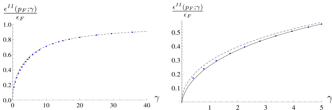
Figure 12: Maximum of the type II spectrum, \epsilon^{II}(p_F; \gamma) , in units of the Fermi energy \epsilon_F , as a function of the dimensionless interaction strength \gamma . The left panel shows the first order approximation in Eq. (51) taking f_2 = 0 (dashed), compared to exact numerics (blue dots). The right panel shows a zoom close to the origin and the second order approximation (solid, black). The agreement is significantly improved when using this correction.
