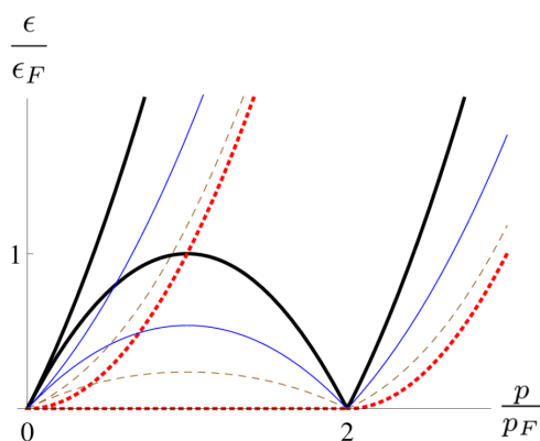
Figure 9: Type I and type II spectra for several values of the interaction strength, from the non-interacting Bose gas (red, dashed) [122] to the Tonks-Girardeau regime (black, solid, thick) with intermediate values \alpha = 0.6 (brown, dashed) and \alpha = 2 (blue, solid).
