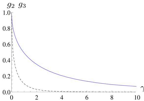
Figure 5: Dimensionless correlation functions g_2 (blue, solid) from Eqs. (10) and (24) and g_3 from Ref. [107] (black, dashed) as functions of the dimensionless interaction strength \gamma . Three-body processes are strongly suppressed at high interaction strength but become of the same order of magnitude as two-body processes in the quasi-condensate regime.
