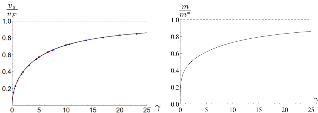
Figure 10: Left panel: dimensionless sound velocity v_s/v_F , where v_F is the Fermi velocity, as a function of the dimensionless Lieb parameter \gamma , numerical (blue dots), numerical from literature [25, 34] (red squares), and our result (black, solid). The Tonks-Girardeau limit is indicated in dashed blue line in both panels. Right panel: dimensionless inverse renormalized mass m/m^* obtained with Eqs. (50), (48), (23) and (10), as a function of the dimensionless Lieb parameter \gamma (black).
