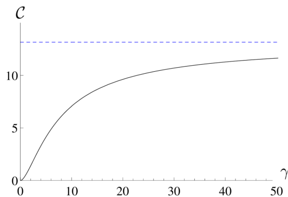
Figure 7: Dimensionless Tan's contact \mathcal{C} as a function of dimensionless interaction strength \gamma (solid, black) and its value in the Tonks-Girardeau limit, \mathcal{C}^{TG} = 4\pi^2/3 (dashed, blue).
