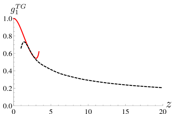
Figure 6: Dimensionless one-body correlation function g_1^{TG} in the Tonks-Girardeau regime as a function of the dimensionless distance z . Short-distance asymptotics given by Eq. (33) (red, solid) and long-distance asymptotics given by Eq. (32) (black, dashed).
