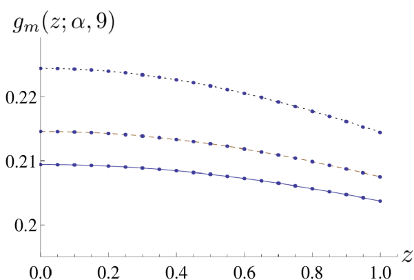
Figure 1: Dimensionless function g_m(z; \alpha, 9) , mean of the 18 th and 20 th order in 1/\alpha of g(z; \alpha) , as a function of the dimensionless variable z , at dimensionless parameters \alpha = 2.5 (solid, blue), \alpha = 2.3 (dashed, brown) and \alpha = 2 (dotted, black) from bottom to top, compared to the corresponding numerically exact solutions (blue dots). Only a few numerical values are shown to improve the visibility, and numerical error is within the size of the dots.
