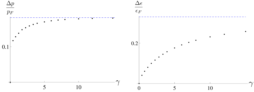
Figure 11: Upper bounds for the validity range in dimensionless momentum (left panel) and dimensionless energy (right panel) around the umklapp point p = 2p_F, \epsilon = 0 of the Luttinger liquid prediction for the excitation spectrum \epsilon^{II} , as functions of the dimensionless interaction strength \gamma . Dots represent the numerical estimate at finite interaction strength, the blue dashed curve is the exact result in the Tonks-Girardeau regime \Delta\epsilon^{TG}/\epsilon_F \simeq 0.330581 and \Delta p^{TG}/p_F \simeq 0.18182
