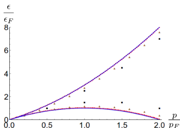
Figure 8: Excitation energy of the Tonks-Girardeau gas \epsilon in units of the Fermi energy in the thermodynamic limit \epsilon_F = \frac{\hbar^2 \pi^2 N^2}{2mL^2} , as a function of the excitation momentum p , in units of the the Fermi momentum in the thermodynamic limit p_F = \frac{\hbar \pi N}{L} , for N = 4 (black squares), N = 10 (brown triangles), N = 100 (red dots). The last one is quasi-indistinguishable from the excitation spectra in the thermodynamic limit (solid, blue).
