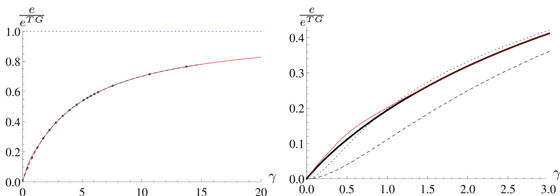
Figure 3: Left panel: dimensionless ground state energy per particle e normalized to its value in the Tonks-Girardeau limit e^{TG} (dotted, blue), as a function of the dimensionless interaction strength \gamma : conjectural expansion at large \gamma (solid, red) as given by Eq. (23) to sixth order, small \gamma expansion (black, dashed) as given by Eq. (10) and numerics (blue points). Right panel: zoom in the weakly-interacting region. Numerically exact result (black, thick) is compared to e_0 (black, dashed), e_0 + e_1 (black, dotted) and the sixth-order expansion (red) in Eq. (23).
