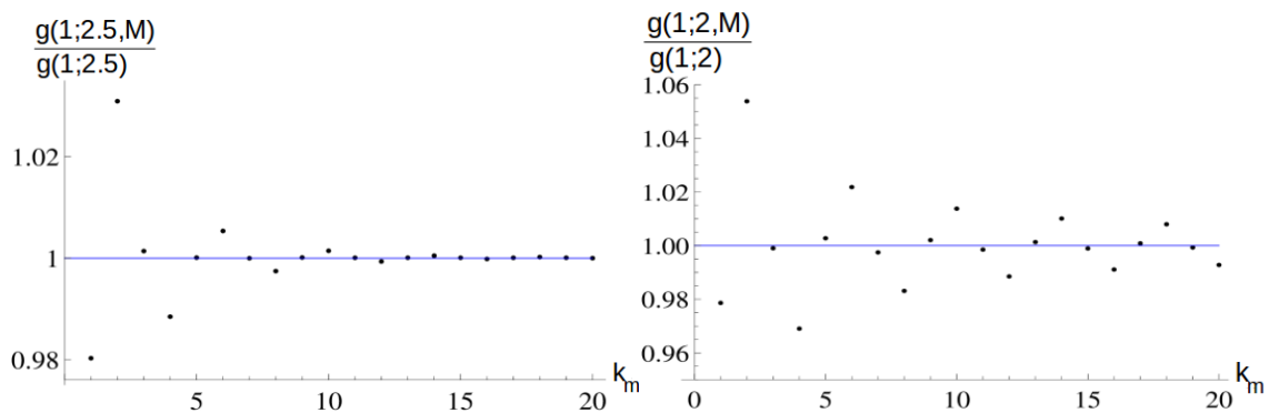
Figure 14: Dimensionless ratio g(1; \alpha, M)/g(1; \alpha) of the approximate analytical solution and the numerically exact solution of Eq. (4) for several values of the maximal order of expansion k_m , at dimensionless parameters \alpha = 2.5 \leftrightarrow \gamma = 6.0257 (left panel) and \alpha = 2 \leftrightarrow \gamma_c = 4.5268 (right panel). The ratio 1 corresponds to the exact solution and is indicated by the blue line as a guide to the eye. When \alpha is decreased, larger values of the parameter M , or equivalently k_m (\leq 2M + 2) , are needed to reach a given accuracy. Quite remarkably, due to the oscillation of the analytics around the exact solution, odd-order terms are more accurate than even ones.
