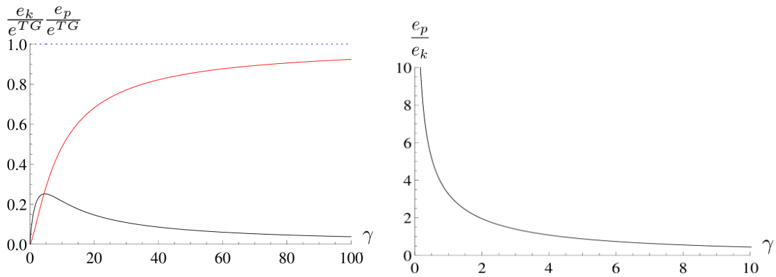
Figure 4: Left panel: dimensionless ground-state kinetic energy per particle (red) and interaction energy per particle (black), normalized to the total energy per particle in the Tonks-Girardeau limit e^{TG} , as a function of the dimensionless interaction strength \gamma . The horizontal line (blue, dotted) is a guide to the eye. Right panel: dimensionless ratio of the interaction and kinetic energy as a function of \gamma .
