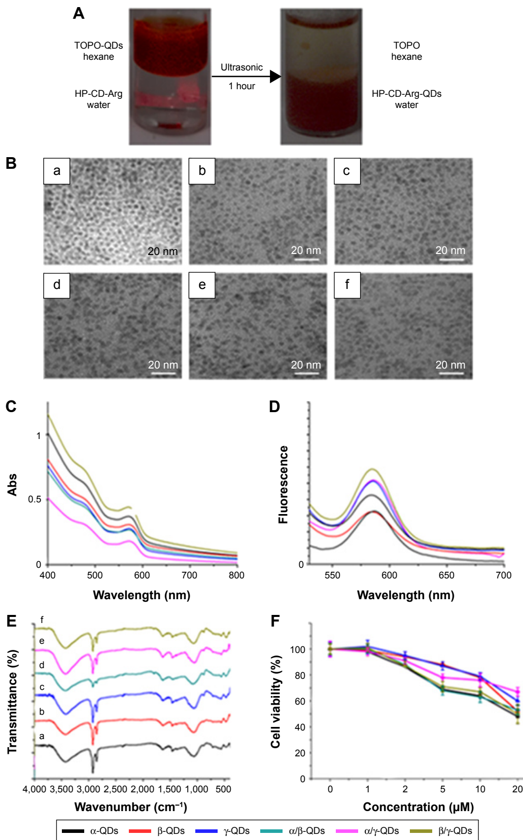
Figure 2 (A) Images of phase transfer reaction for the synthesis of \alpha -QDs triggered by ultrasound treatment; the reaction phenomenon for the other QD nanocarriers was similar. (B) TEM images of (a) \alpha -QDs, (b) \beta -QDs, (c) \gamma -QDs, (d) \alpha/\beta -QDs, (e) \alpha/\gamma -QDs, and (f) \beta/\gamma -QDs. (C) The UV-visible spectra of QD nanocarriers. (D) Fluorescence emission spectra of QD nanocarriers; Ex: 488 nm. (E) FT-IR spectra of QD nanocarriers. (F) Cytotoxicity of QD nanocarriers in A549 cells after 72 hours, as determined by MTT.
