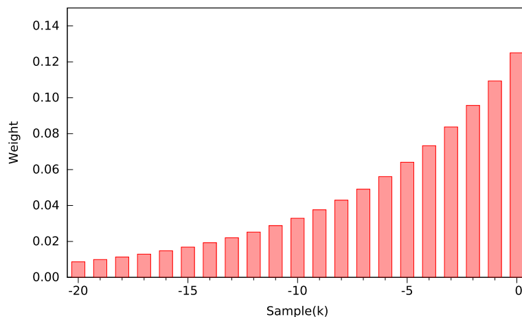
Fig. 3 Example of EMA over a past window of size n = 20 , where less weight is given to old samples when computing the mean in each measure
