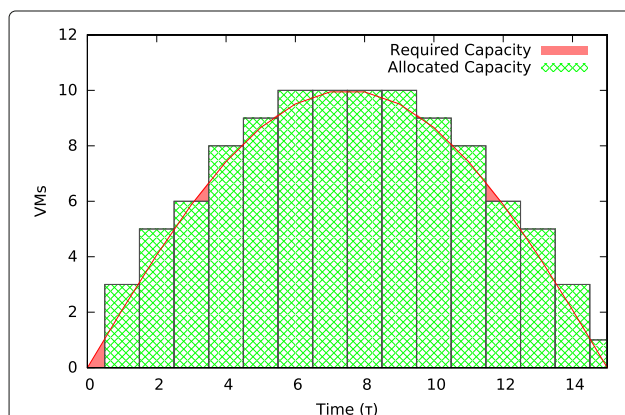
Fig. 1 The actual capacity demand has to be quantized at a resolution determined by the capacity of the smallest VM available for provisioning. Overallocation means an opportunity cost, underallocation means lost revenue
