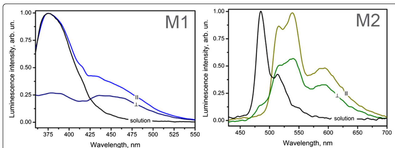
Fig. 7 Photoluminescence spectra of M1 and M2 deposited on SnO 2 -coated glass with parallel and perpendicular applied electric field. Spectra of M1 and M2 chloroform solutions are shown for comparison
