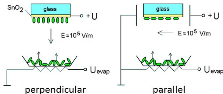
Fig. 2 Schemes of electric field application for controlling the spatial orientation of organic molecules perpendicularly and in parallel to the surface
