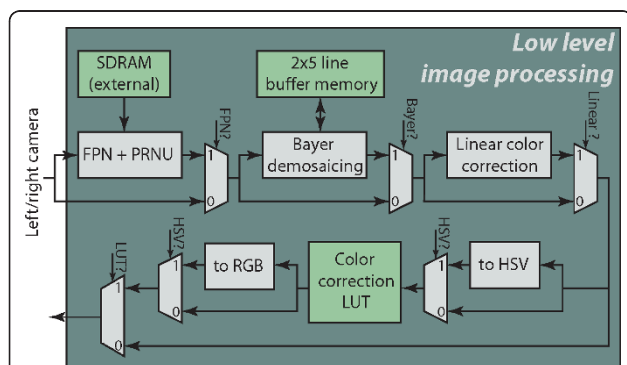
Figure 2 FPGA pipeline of low-level image processing. Only the fixed pattern noise removal and pixel response non-uniformity equalization need access to external memory.
