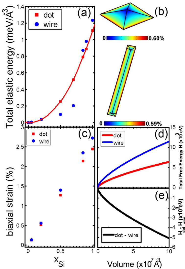
Figure 10 FE simulations. (a) Total elastic energy of wires and dots as a function of the Si content. (b) Three-dimensional maps of biaxial strain for pyramidal dots and wires for a Si content of 10%. (c) Average biaxial strain for wires and dots as a function of the Si content. (d) Total strain + surface energy for wires and dots as a function of volume. (e) Relative difference of the curves shown in (d).
