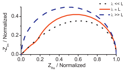
Fig. 2. Possible impedance spectrum shapes for \alpha_r = 1 in Eq. (5) of the porous electrode theory of Levie response.
