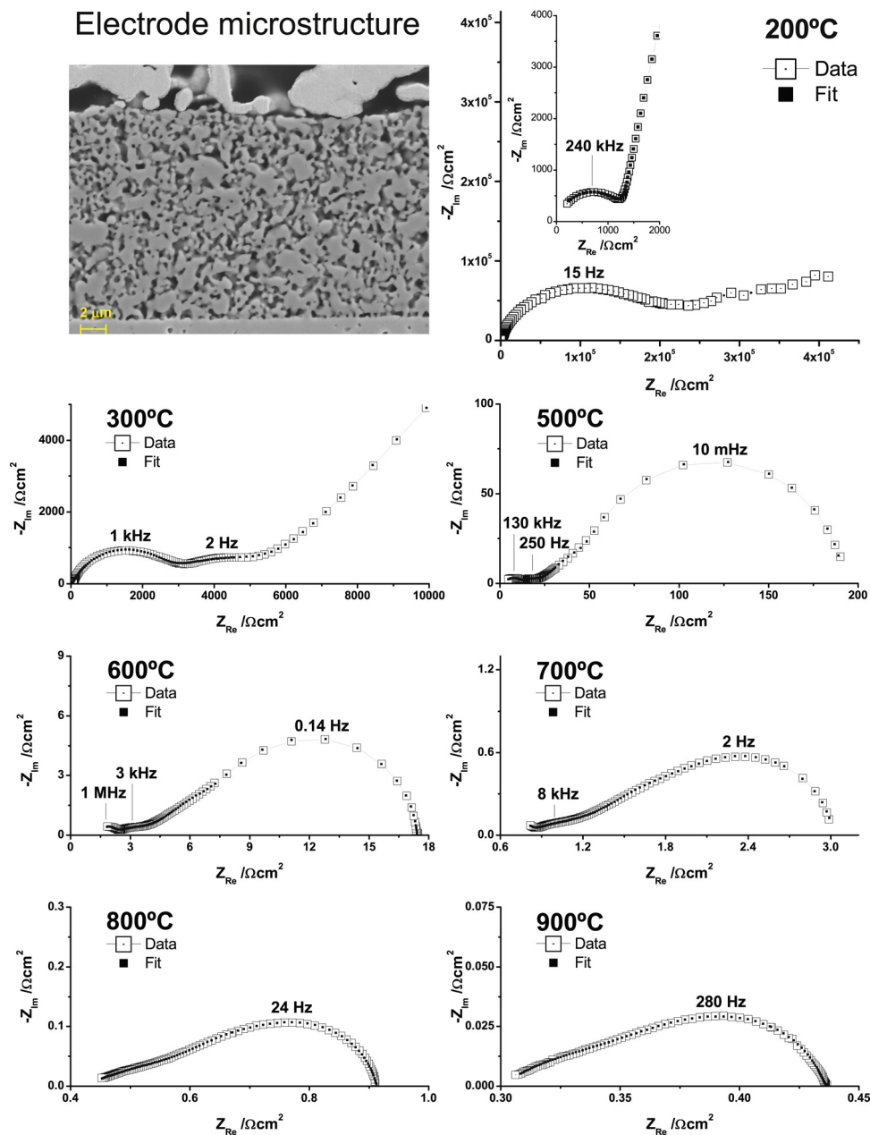
Fig. 7. Impedance spectra in the temperature range 200–900 °C of a LSM:YSZ composite cathode on a CGO electrolyte sintered at 1180 °C. The impedance spectra in the temperature range 300–700 °C has been fitted with the equivalent circuit (RQ)_1-(RQ)_2 -PET, while the spectra above 700 °C has been fitted with the equivalent circuit (RQ)_2 -PET.
