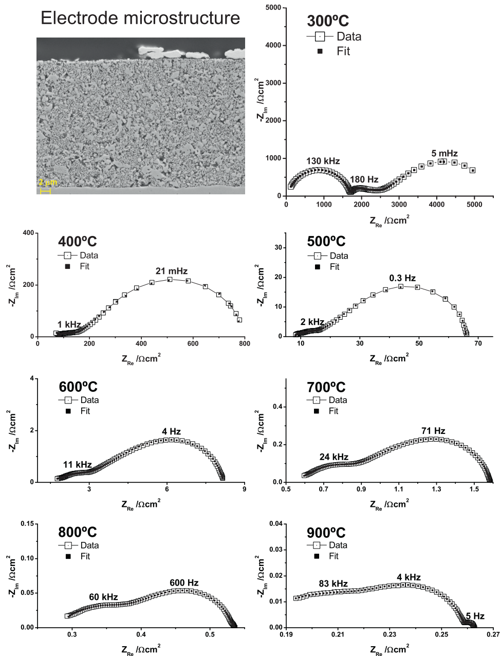
Fig. 5. Impedance spectra in the temperature range 300–900 °C of a LSM:YSZ composite cathode on a YSZ electrolyte sintered at 1080 °C. The low temperature spectra have been fitted with the equivalent circuit (RQ)_1-(RQ)_2-(RQ)_3 -PET, while the high temperature spectra >800 °C has been fitted with the equivalent circuit R_s(RQ)_3 -PET-FLW.
