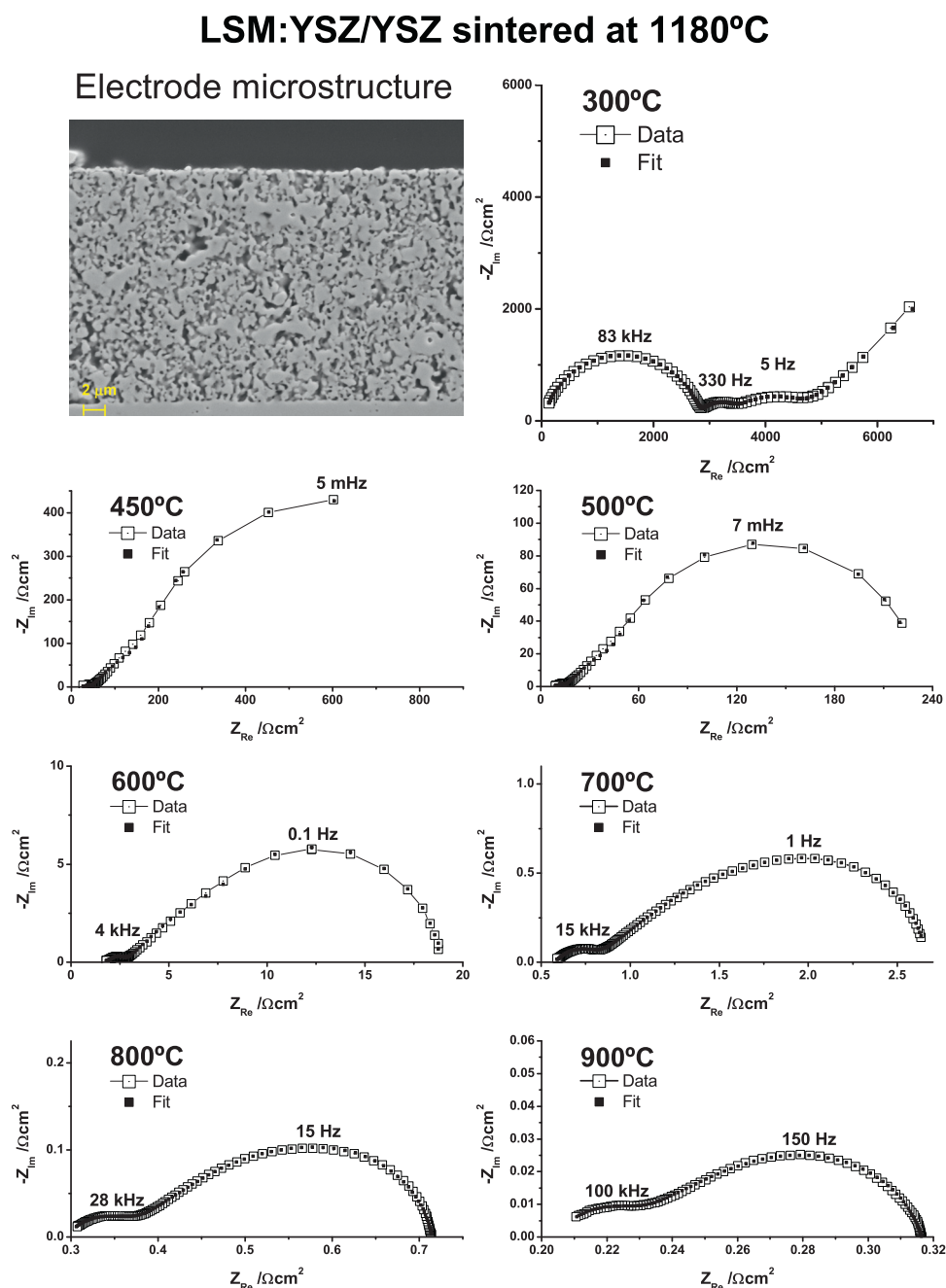
Fig. 3. Impedance spectra in the temperature range 300–900 °C of a LSM:YSZ composite cathode on a YSZ electrolyte sintered at 1180 °C. The impedance has been fitted with the equivalent circuit (RQ)_1-(RQ)_2-(RQ)_3 -PET at low temperatures and R_s(RQ)_3 -PET at high temperatures.
