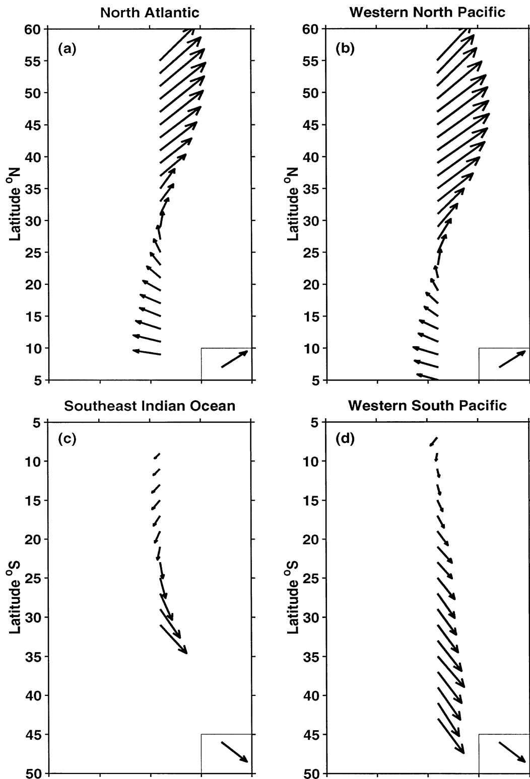
FIG. 3. Average motion of tropical cyclones vs latitude during 1970–99 from best-track data. The reference arrow has zonal and meridional components of 5 m s -1 .
