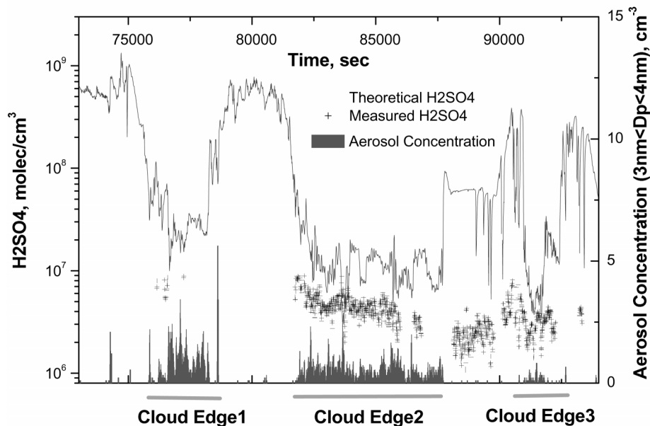
FIG. 5. Time series of three cloud-edge passes from PEM-Tropics B where recent nucleation can be seen in the 3–4-nm particle concentrations when measured sulfuric acid (+) approaches concentration needed for classical binary nucleation (line).
