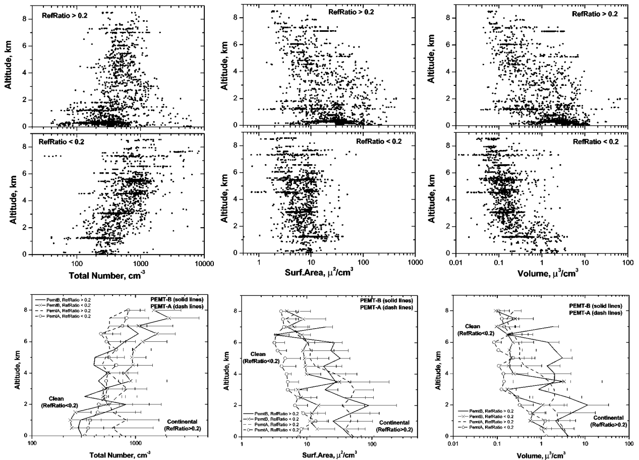
FIG. 14. Vertical profiles number, surface area, and volume integrated from aerosol size distribution data and coded with RefRatio to reveal typical range clean and “perturbed” aerosol measured over the Pacific on PEM-Tropics A and B. High RefRatio generally indicates continental pollution plumes (soot and dust).
