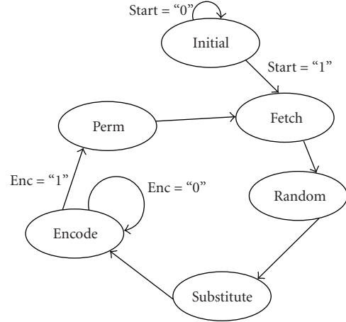
FIGURE 9: Control unit as a Finite State Machine (FSM).
