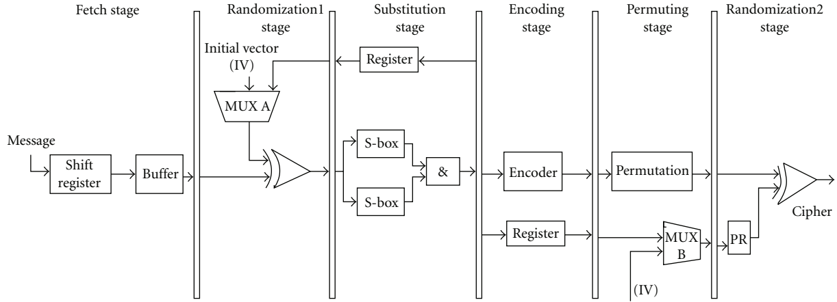
FIGURE 10: Architecture of the pipelined ECBC datapath.
